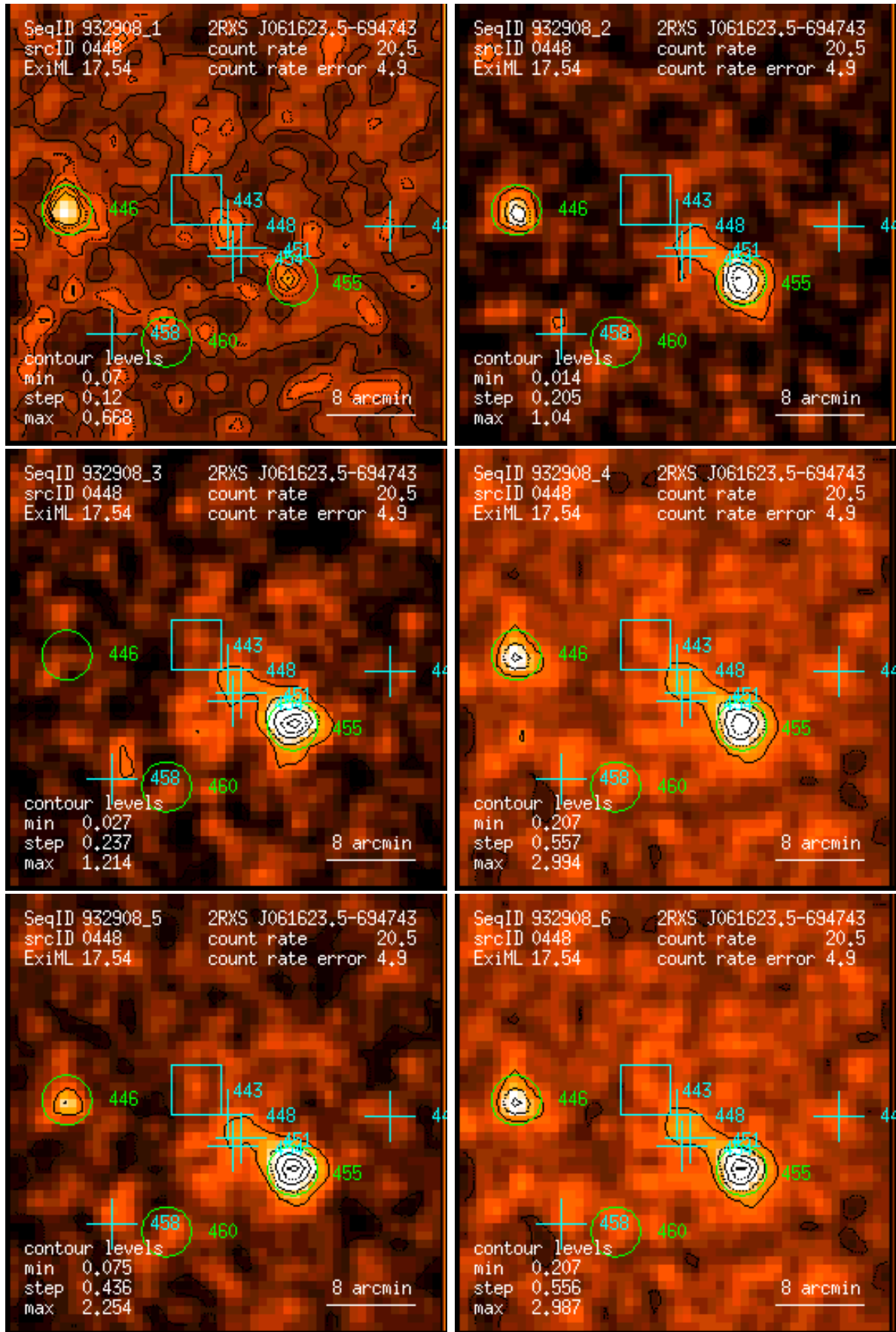
Figure 448: RASS 932908: detection 0448: band rate images, Gaussian filter: (1) PSPC channels 11 – 41, (2) 52 – 90, (3) 91 – 201, (4) 11 – 235, (5) 52 – 201, (6) 11 – 201. Broad band rates in counts/ks. Band rate contour levels in counts/ks/arcmin 2 .
