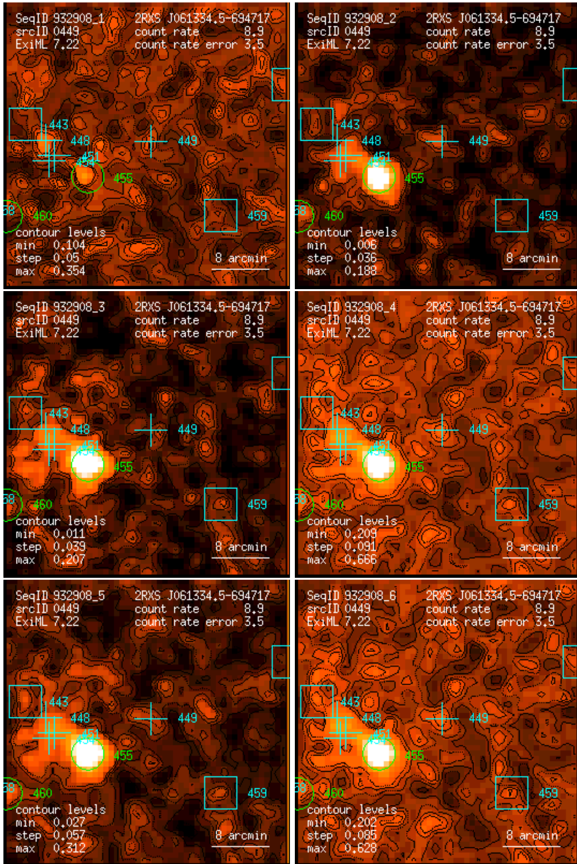
Figure 449: RASS 932908: detection 0449: band rate images, Gaussian filter: (1) PSPC channels 11 – 41, (2) 52 – 90, (3) 91 – 201, (4) 11 – 235, (5) 52 – 201, (6) 11 – 201. Broad band rates in counts/ks. Band rate contour levels in counts/ks/arcmin 2 .
