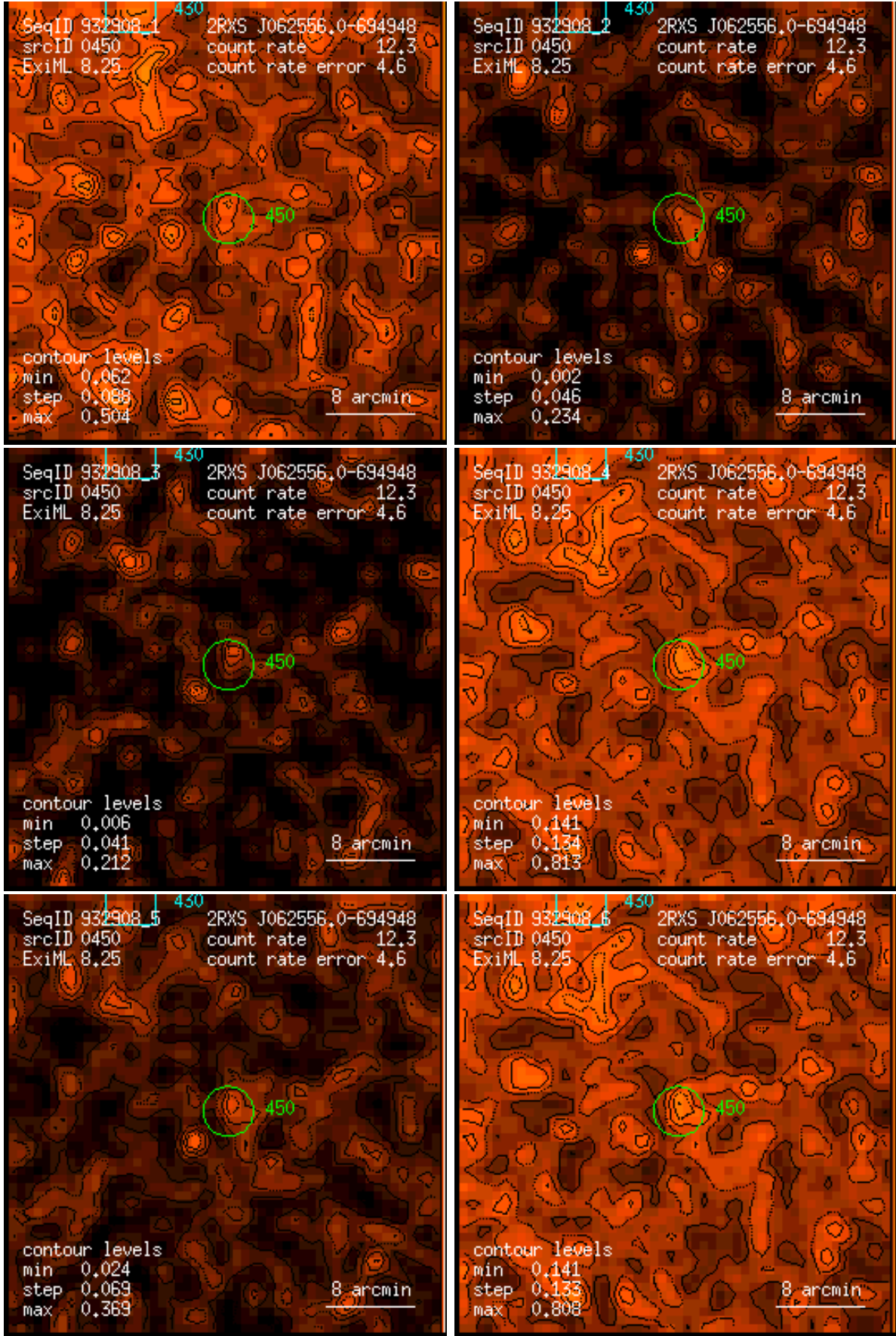
Figure 450: RASS 932908: detection 0450: band rate images, Gaussian filter: (1) PSPC channels 11 – 41, (2) 52 – 90, (3) 91 – 201, (4) 11 – 235, (5) 52 – 201, (6) 11 – 201. Broad band rates in counts/ks. Band rate contour levels in counts/ks/arcmin 2 .
