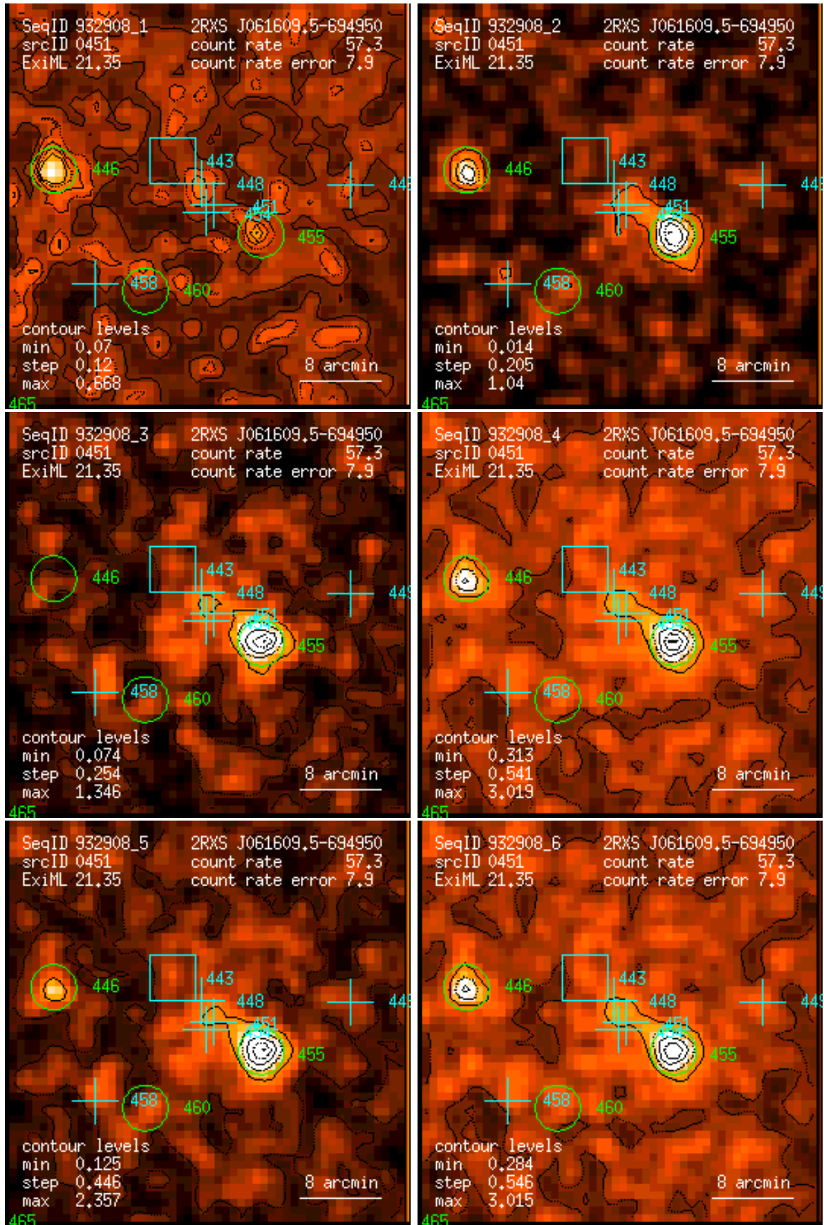
Figure 451: RASS 932908: detection 0451: band rate images, Gaussian filter: (1) PSPC channels 11 – 41, (2) 52 – 90, (3) 91 – 201, (4) 11 – 235, (5) 52 – 201, (6) 11 – 201. Broad band rates in counts/ks. Band rate contour levels in counts/ks/arcmin 2 .
