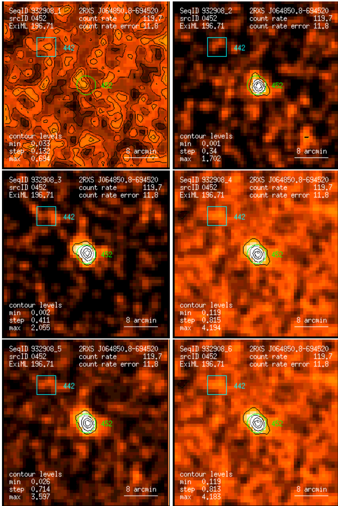
Figure 452: RASS 932908: detection 0452: band rate images, Gaussian filter: (1) PSPC channels 11 – 41, (2) 52 – 90, (3) 91 – 201, (4) 11 – 235, (5) 52 – 201, (6) 11 – 201. Broad band rates in counts/ks. Band rate contour levels in counts/ks/arcmin 2 .
