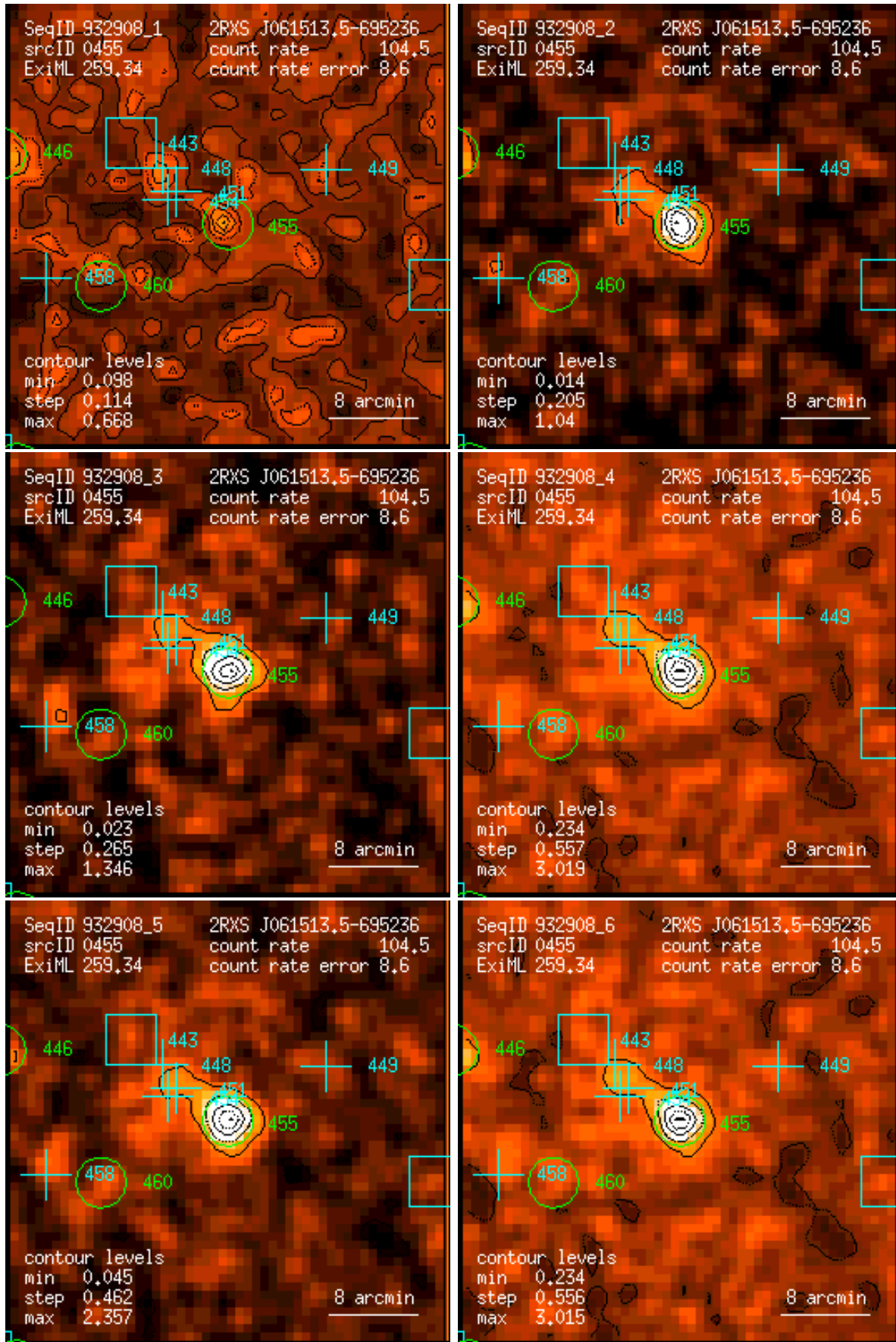
Figure 455: RASS 932908: detection 0455: band rate images, Gaussian filter: (1) PSPC channels 11 – 41, (2) 52 – 90, (3) 91 – 201, (4) 11 – 235, (5) 52 – 201, (6) 11 – 201. Broad band rates in counts/ks. Band rate contour levels in counts/ks/arcmin 2 .
