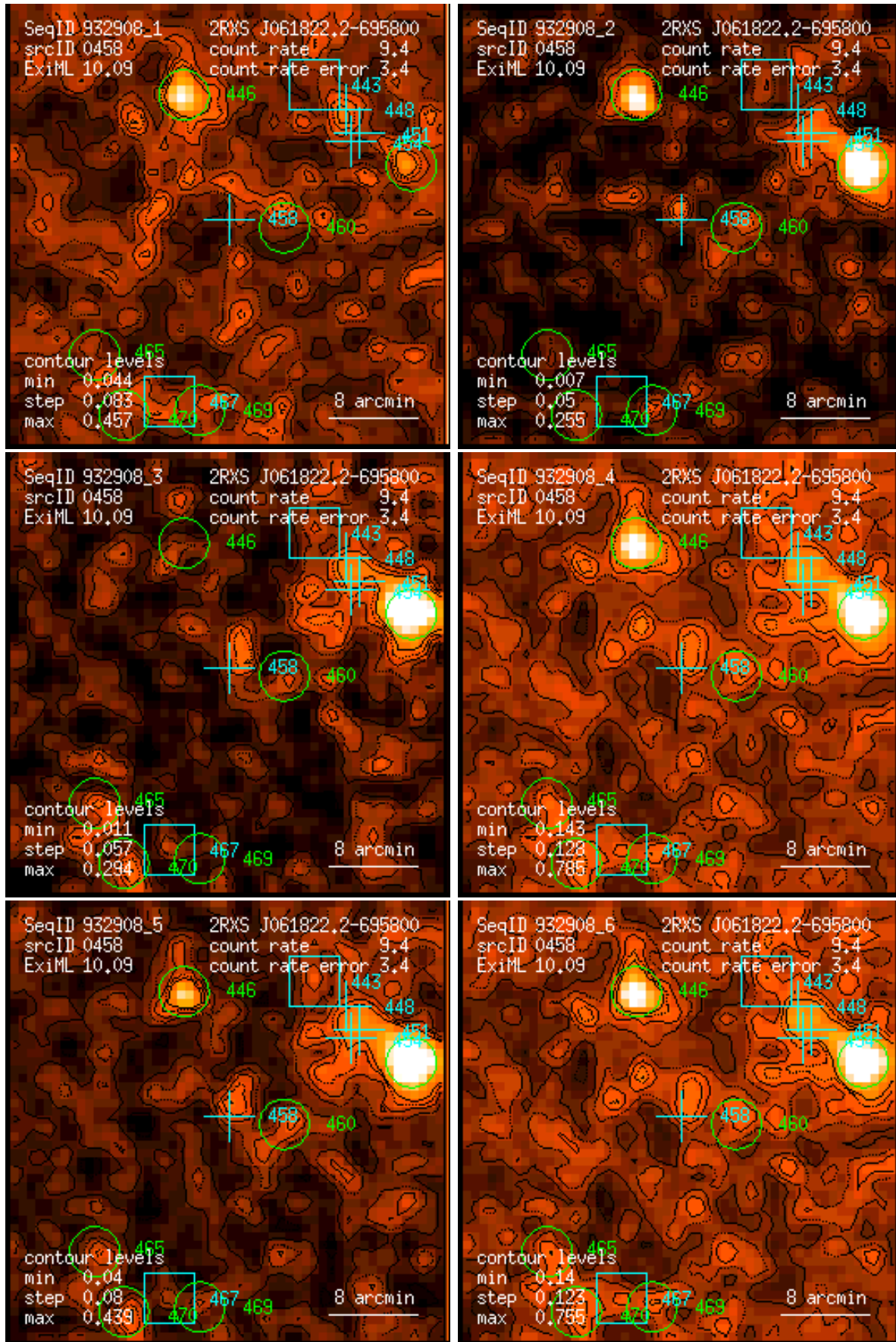
Figure 458: RASS 932908: detection 0458: band rate images, Gaussian filter: (1) PSPC channels 11 – 41, (2) 52 – 90, (3) 91 – 201, (4) 11 – 235, (5) 52 – 201, (6) 11 – 201. Broad band rates in counts/ks. Band rate contour levels in counts/ks/arcmin 2 .
