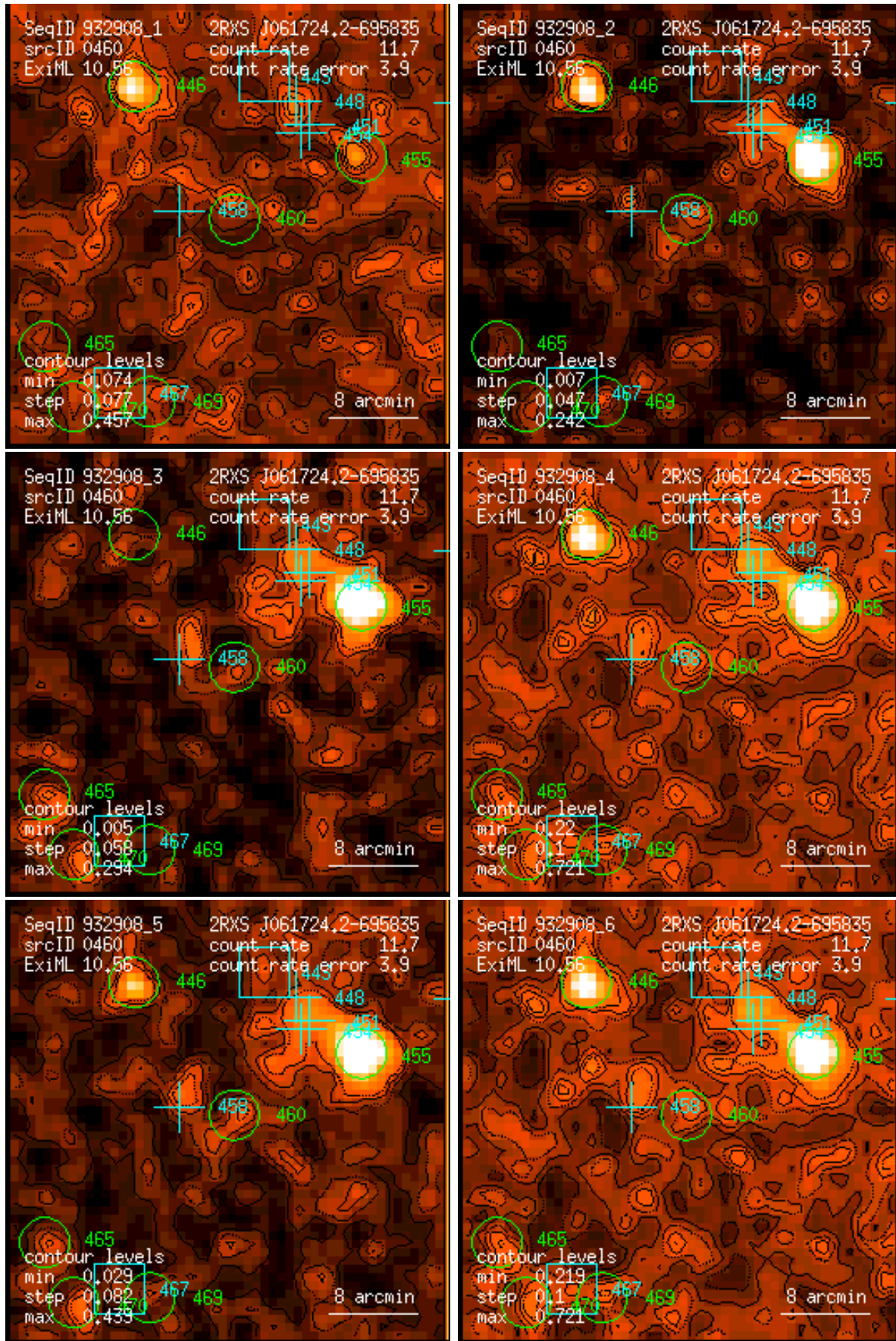
Figure 460: RASS 932908: detection 0460: band rate images, Gaussian filter: (1) PSPC channels 11 – 41, (2) 52 – 90, (3) 91 – 201, (4) 11 – 235, (5) 52 – 201, (6) 11 – 201. Broad band rates in counts/ks. Band rate contour levels in counts/ks/arcmin 2 .
