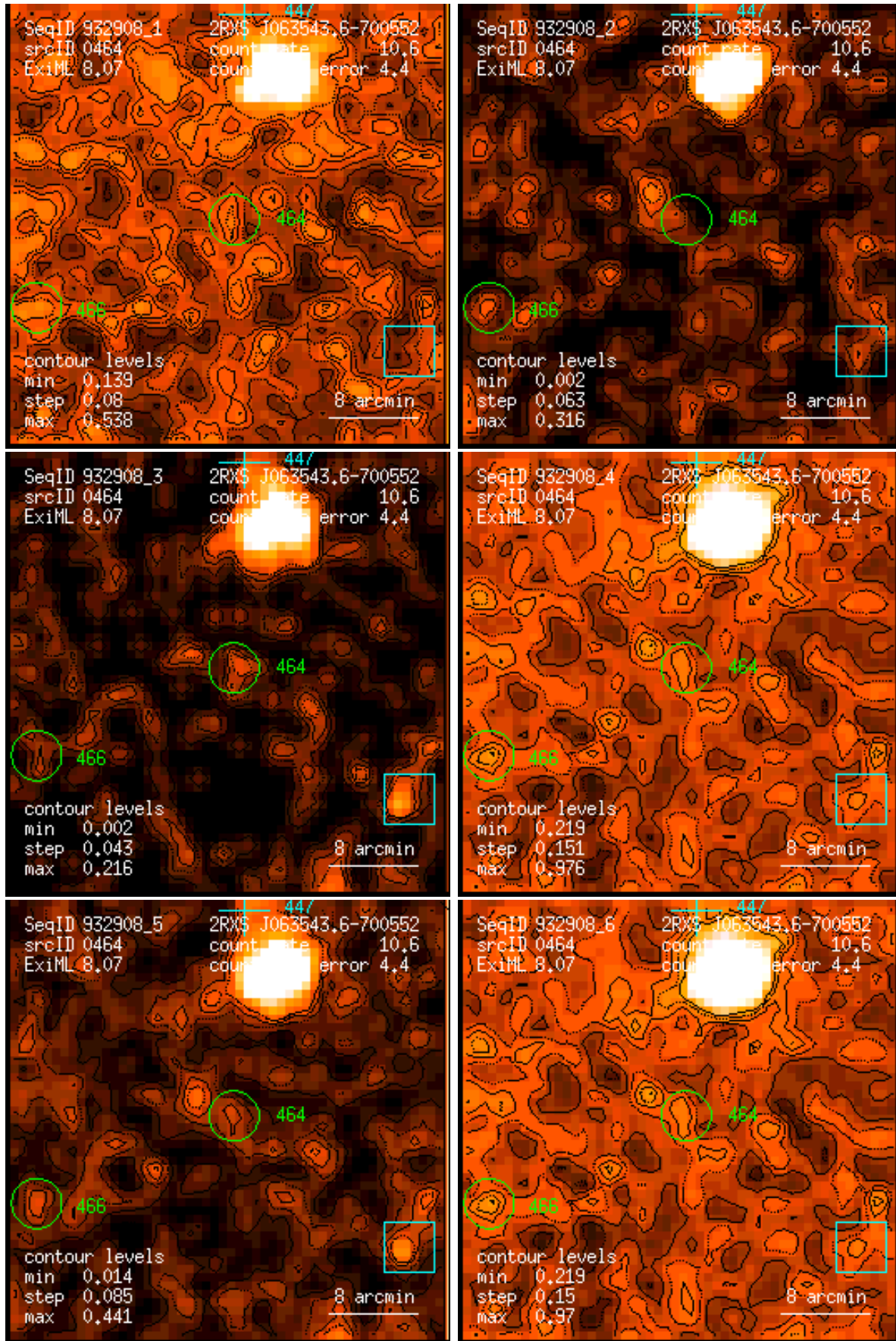
Figure 464: RASS 932908: detection 0464: band rate images, Gaussian filter: (1) PSPC channels 11 – 41, (2) 52 – 90, (3) 91 – 201, (4) 11 – 235, (5) 52 – 201, (6) 11 – 201. Broad band rates in counts/ks. Band rate contour levels in counts/ks/arcmin 2 .
