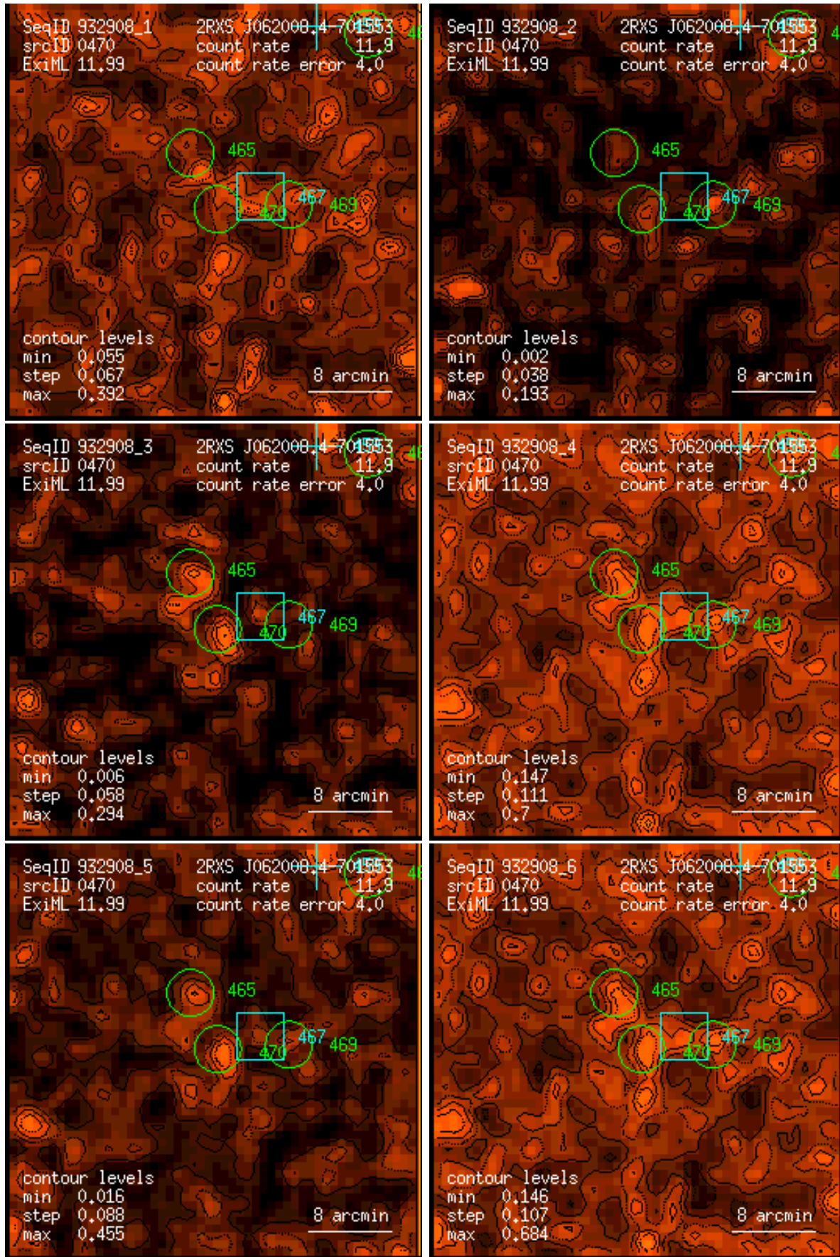
Figure 470: RASS 932908: detection 0470: band rate images, Gaussian filter: (1) PSPC channels 11 – 41, (2) 52 – 90, (3) 91 – 201, (4) 11 – 235, (5) 52 – 201, (6) 11 – 201. Broad band rates in counts/ks. Band rate contour levels in counts/ks/arcmin 2 .
