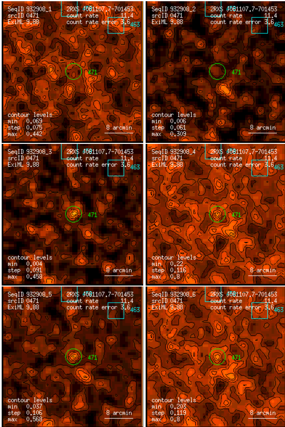
Figure 471: RASS 932908: detection 0471: band rate images, Gaussian filter: (1) PSPC channels 11 – 41, (2) 52 – 90, (3) 91 – 201, (4) 11 – 235, (5) 52 – 201, (6) 11 – 201. Broad band rates in counts/ks. Band rate contour levels in counts/ks/arcmin 2 .
