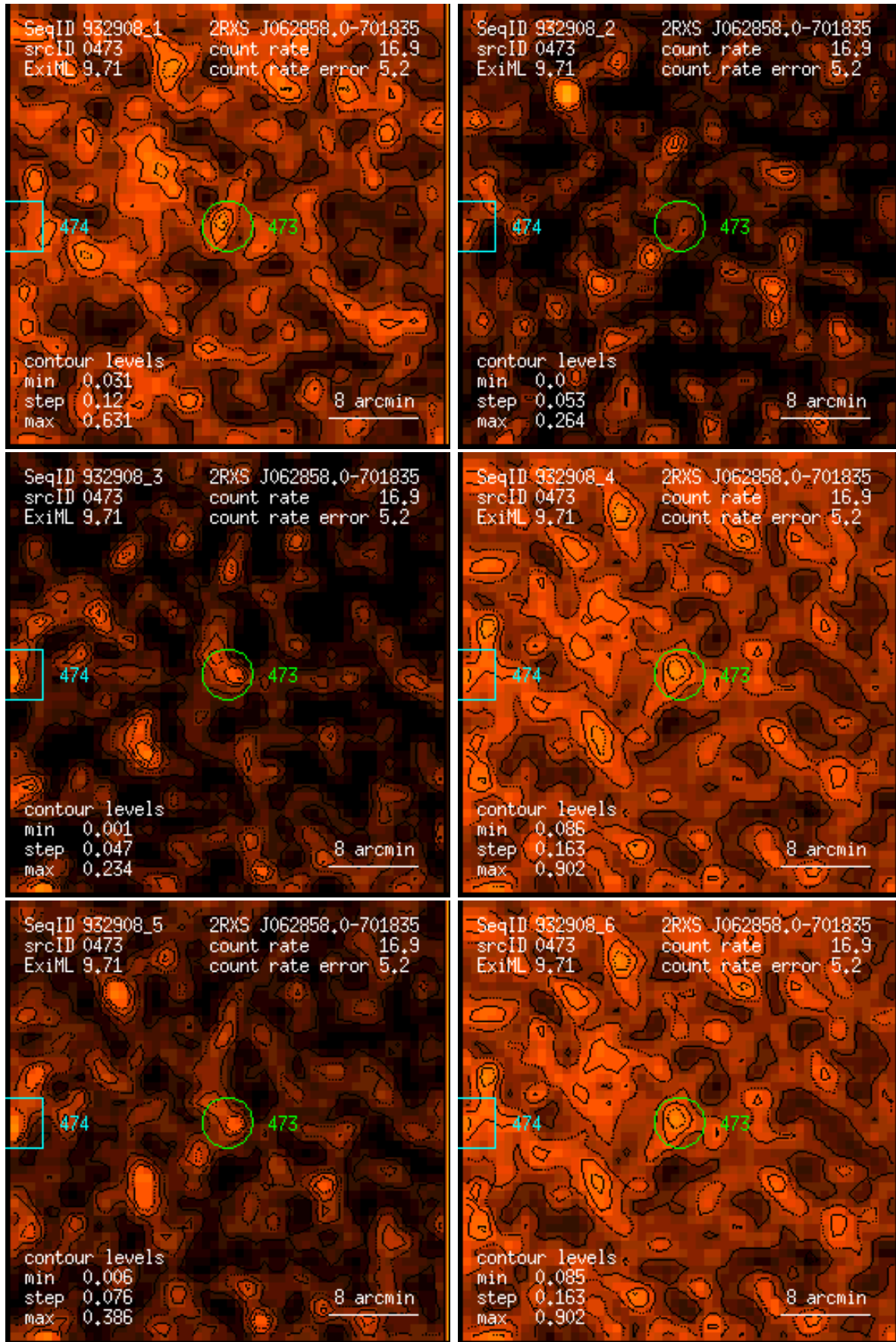
Figure 473: RASS 932908: detection 0473: band rate images, Gaussian filter: (1) PSPC channels 11 – 41, (2) 52 – 90, (3) 91 – 201, (4) 11 – 235, (5) 52 – 201, (6) 11 – 201. Broad band rates in counts/ks. Band rate contour levels in counts/ks/arcmin 2 .
