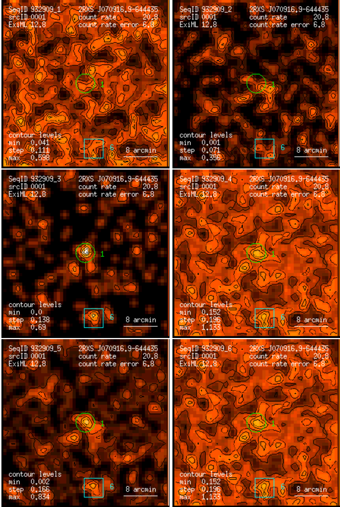
Figure 1: RASS 932909: detection 0001: band rate images, Gaussian filter: (1) PSPC channels 11 – 41, (2) 52 – 90, (3) 91 – 201, (4) 11 – 235, (5) 52 – 201, (6) 11 – 201. Broad band rates in counts/ks. Band rate contour levels in counts/ks/arcmin 2 .
