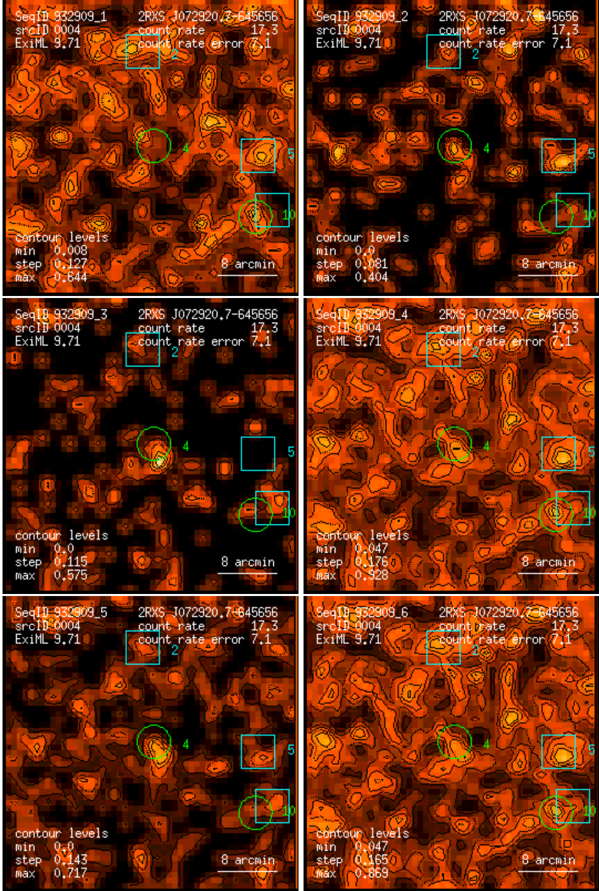
Figure 4: RASS 932909: detection 0004: band rate images, Gaussian filter: (1) PSPC channels 11 – 41, (2) 52 – 90, (3) 91 – 201, (4) 11 – 235, (5) 52 – 201, (6) 11 – 201. Broad band rates in counts/ks. Band rate contour levels in counts/ks/arcmin 2 .
