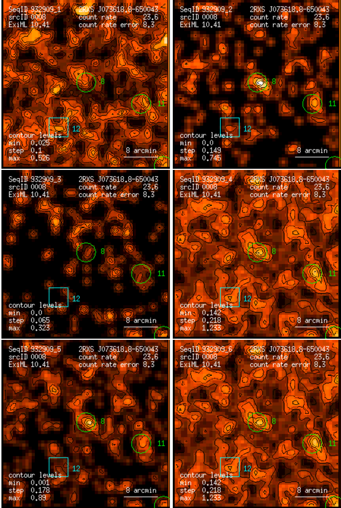
Figure 8: RASS 932909: detection 0008: band rate images, Gaussian filter: (1) PSPC channels 11 – 41, (2) 52 – 90, (3) 91 – 201, (4) 11 – 235, (5) 52 – 201, (6) 11 – 201. Broad band rates in counts/ks. Band rate contour levels in counts/ks/arcmin 2 .
