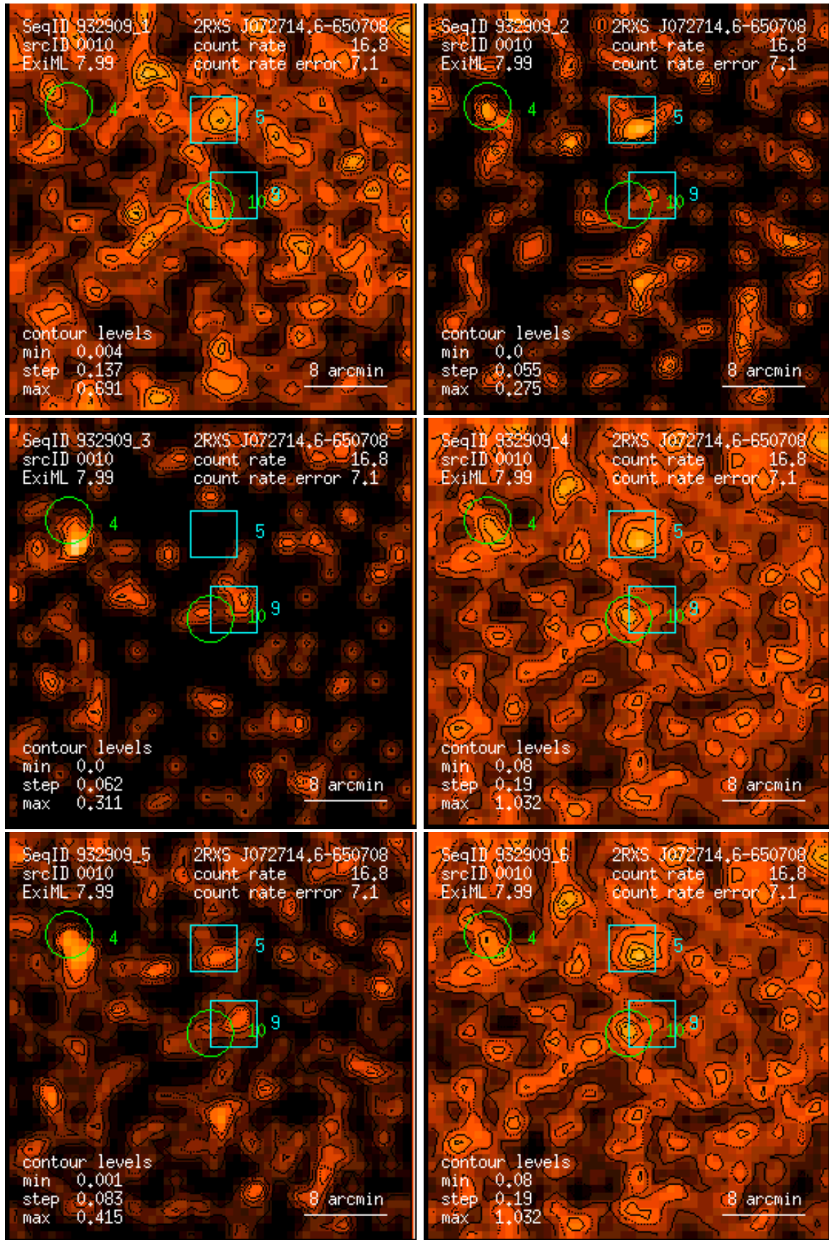
Figure 10: RASS 932909: detection 0010: band rate images, Gaussian filter: (1) PSPC channels 11 – 41, (2) 52 – 90, (3) 91 – 201, (4) 11 – 235, (5) 52 – 201, (6) 11 – 201. Broad band rates in counts/ks. Band rate contour levels in counts/ks/arcmin 2 .
