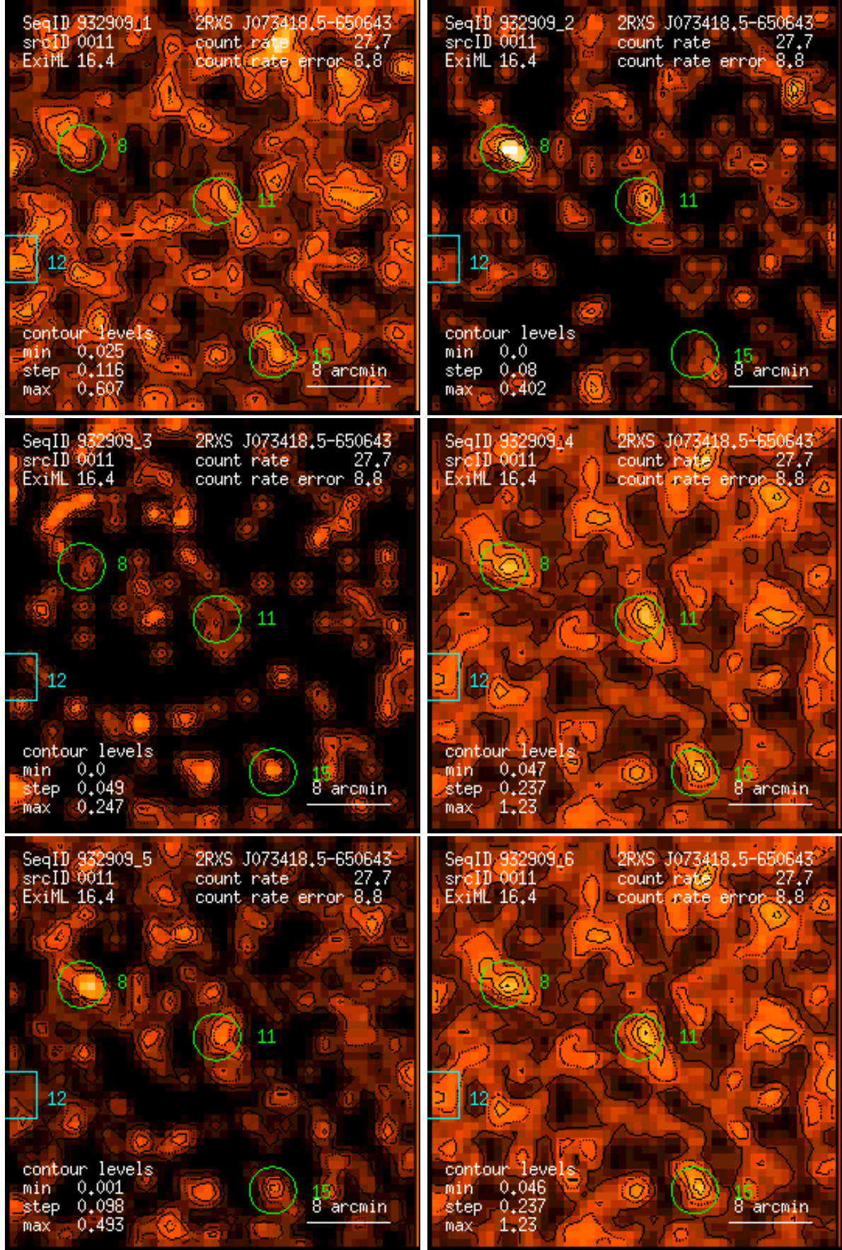
Figure 11: RASS 932909: detection 0011: band rate images, Gaussian filter: (1) PSPC channels 11 – 41, (2) 52 – 90, (3) 91 – 201, (4) 11 – 235, (5) 52 – 201, (6) 11 – 201. Broad band rates in counts/ks. Band rate contour levels in counts/ks/arcmin 2 .
