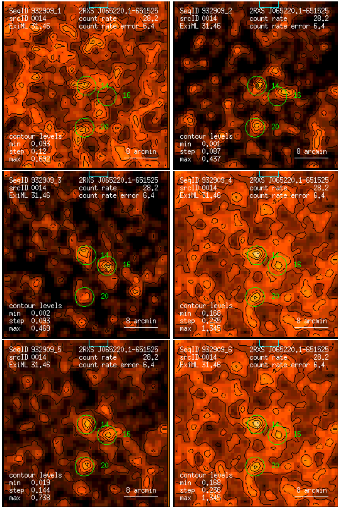
Figure 14: RASS 932909: detection 0014: band rate images, Gaussian filter: (1) PSPC channels 11 – 41, (2) 52 – 90, (3) 91 – 201, (4) 11 – 235, (5) 52 – 201, (6) 11 – 201. Broad band rates in counts/ks. Band rate contour levels in counts/ks/arcmin 2 .
