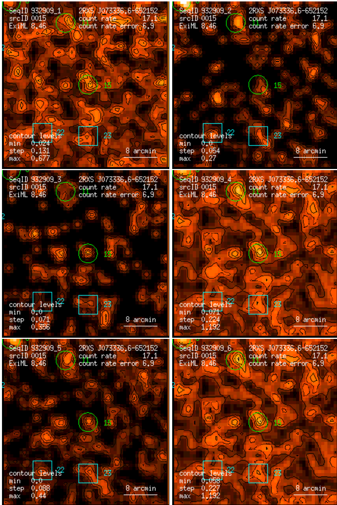
Figure 15: RASS 932909: detection 0015: band rate images, Gaussian filter: (1) PSPC channels 11 – 41, (2) 52 – 90, (3) 91 – 201, (4) 11 – 235, (5) 52 – 201, (6) 11 – 201. Broad band rates in counts/ks. Band rate contour levels in counts/ks/arcmin 2 .
