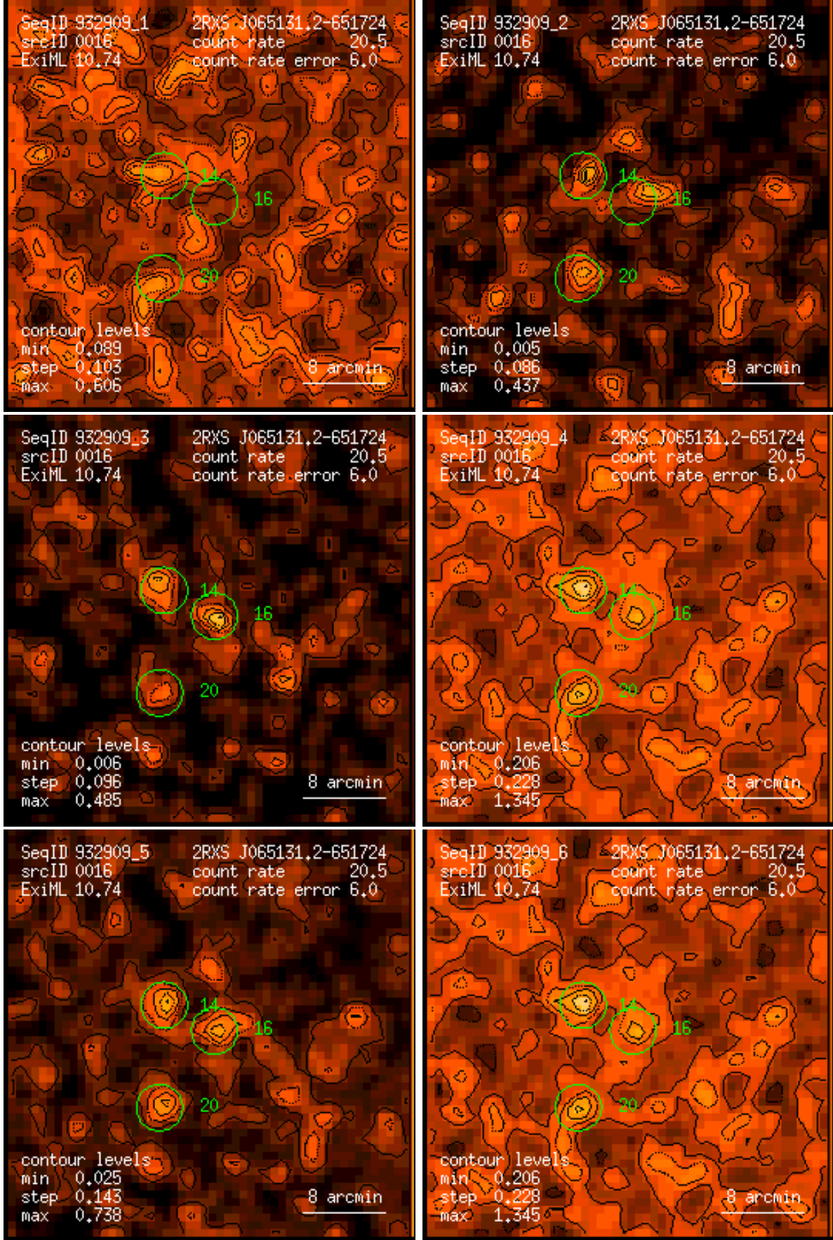
Figure 16: RASS 932909: detection 0016: band rate images, Gaussian filter: (1) PSPC channels 11 – 41, (2) 52 – 90, (3) 91 – 201, (4) 11 – 235, (5) 52 – 201, (6) 11 – 201. Broad band rates in counts/ks. Band rate contour levels in counts/ks/arcmin 2 .
