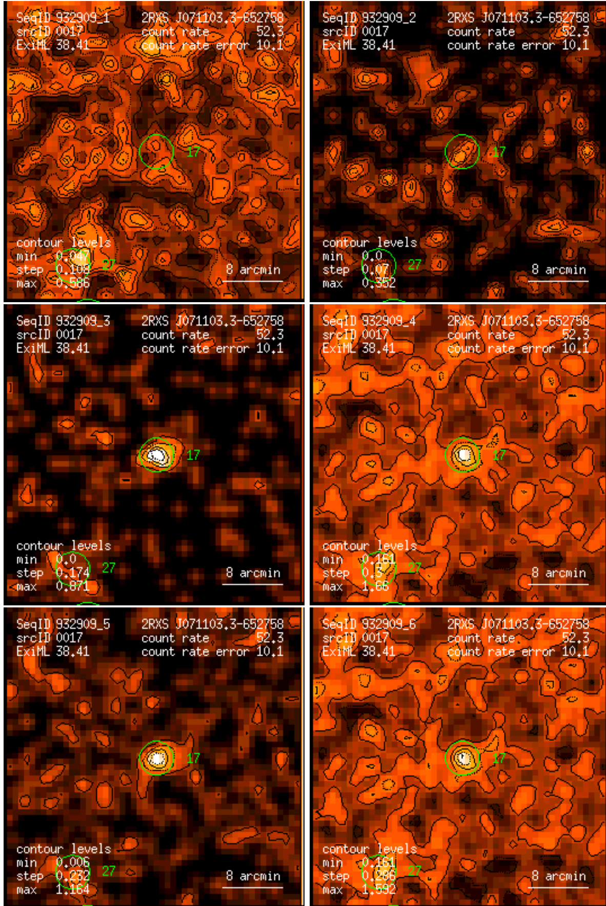
Figure 17: RASS 932909: detection 0017: band rate images, Gaussian filter: (1) PSPC channels 11 – 41, (2) 52 – 90, (3) 91 – 201, (4) 11 – 235, (5) 52 – 201, (6) 11 – 201. Broad band rates in counts/ks. Band rate contour levels in counts/ks/arcmin 2 .
