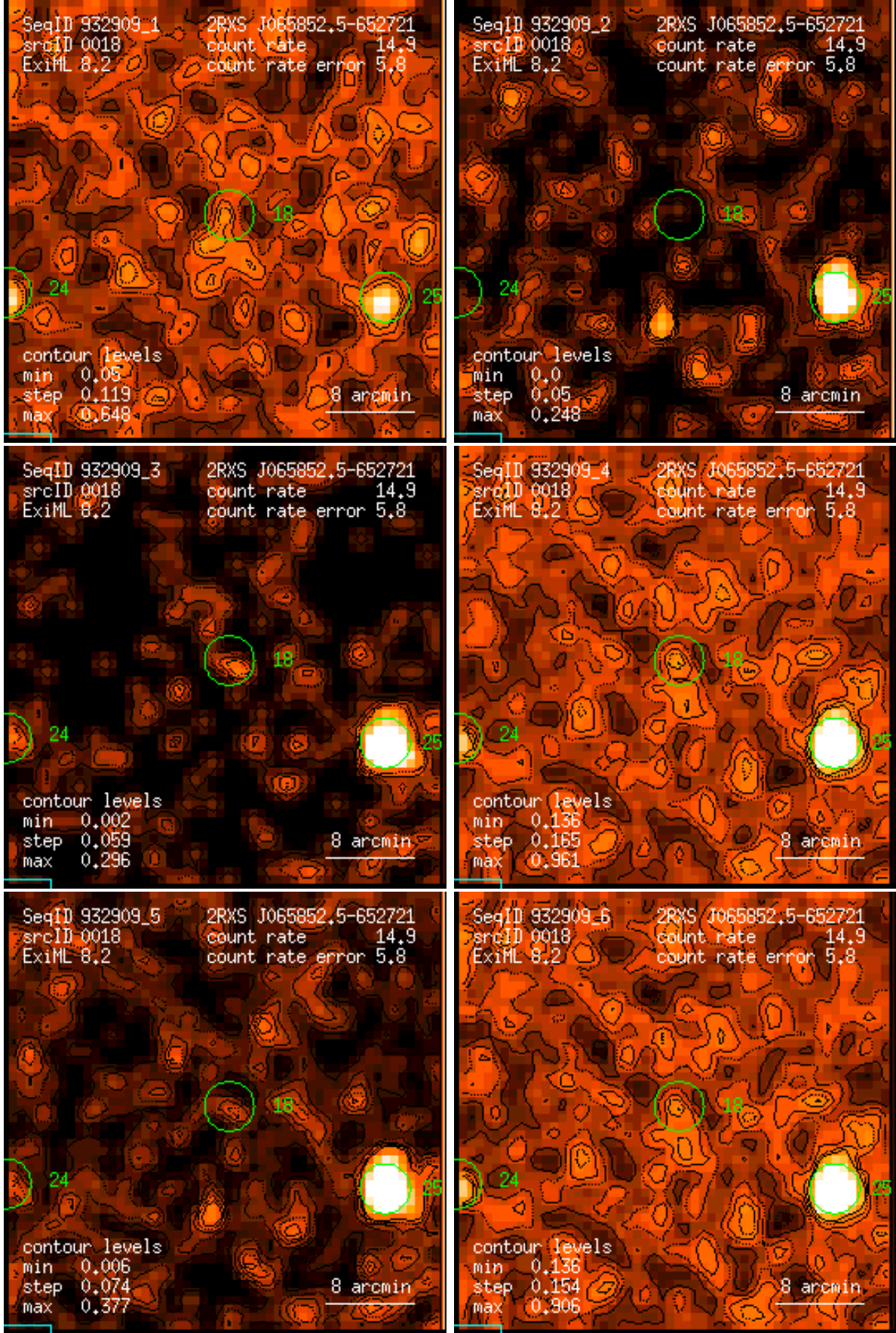
Figure 18: RASS 932909: detection 0018: band rate images, Gaussian filter: (1) PSPC channels 11 – 41, (2) 52 – 90, (3) 91 – 201, (4) 11 – 235, (5) 52 – 201, (6) 11 – 201. Broad band rates in counts/ks. Band rate contour levels in counts/ks/arcmin 2 .
