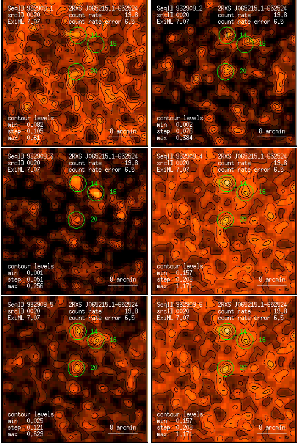
Figure 20: RASS 932909: detection 0020: band rate images, Gaussian filter: (1) PSPC channels 11 – 41, (2) 52 – 90, (3) 91 – 201, (4) 11 – 235, (5) 52 – 201, (6) 11 – 201. Broad band rates in counts/ks. Band rate contour levels in counts/ks/arcmin 2 .
