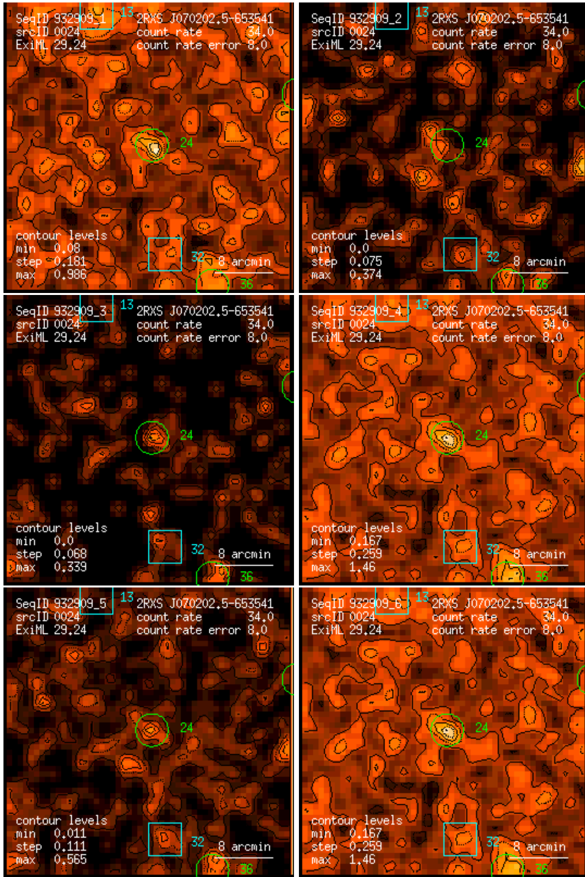
Figure 24: RASS 932909: detection 0024: band rate images, Gaussian filter: (1) PSPC channels 11 – 41, (2) 52 – 90, (3) 91 – 201, (4) 11 – 235, (5) 52 – 201, (6) 11 – 201. Broad band rates in counts/ks. Band rate contour levels in counts/ks/arcmin 2 .
