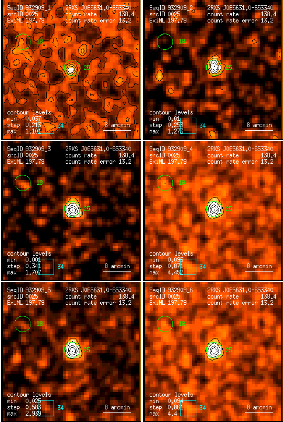
Figure 25: RASS 932909: detection 0025: band rate images, Gaussian filter: (1) PSPC channels 11 – 41, (2) 52 – 90, (3) 91 – 201, (4) 11 – 235, (5) 52 – 201, (6) 11 – 201. Broad band rates in counts/ks. Band rate contour levels in counts/ks/arcmin 2 .
