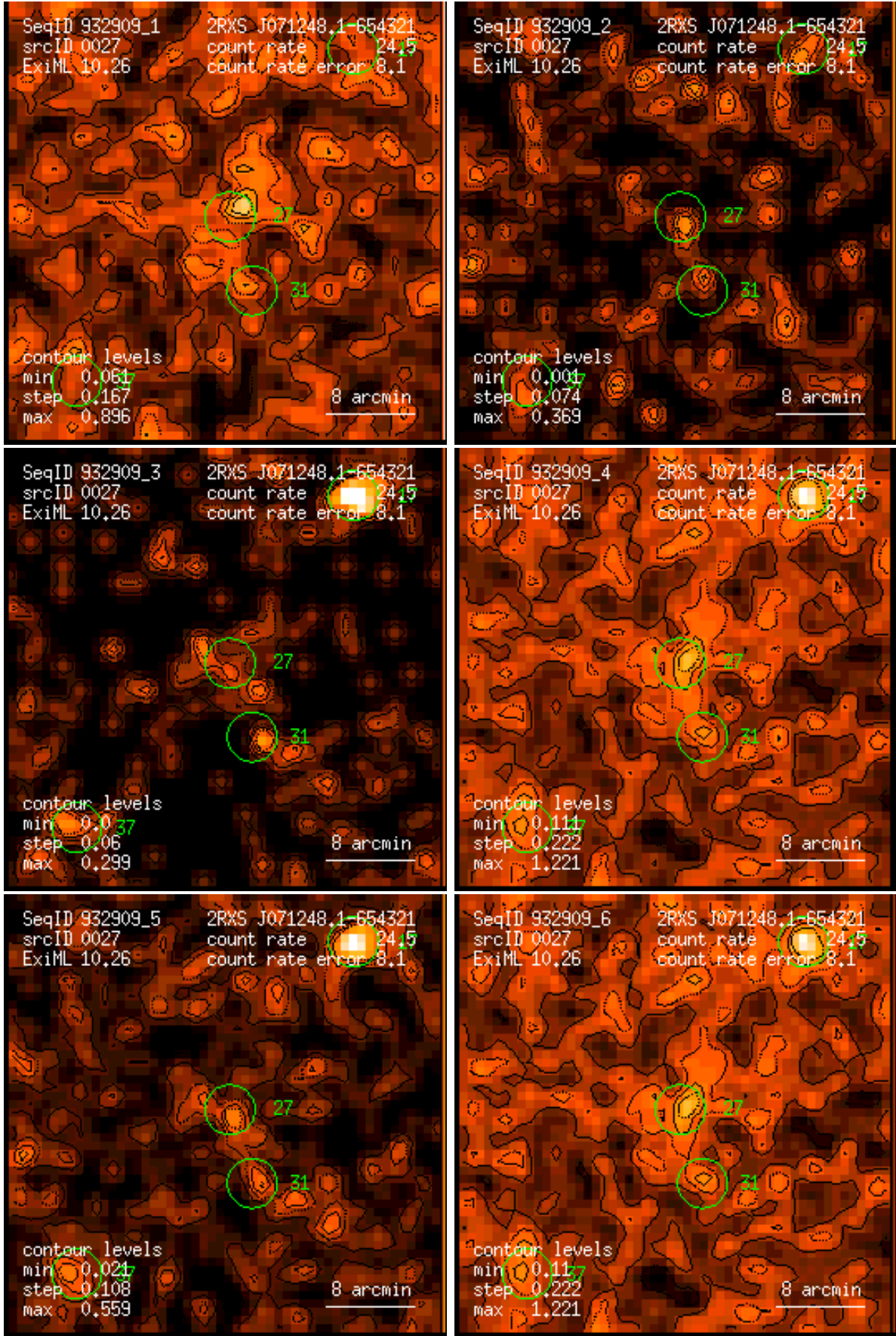
Figure 27: RASS 932909: detection 0027: band rate images, Gaussian filter: (1) PSPC channels 11 – 41, (2) 52 – 90, (3) 91 – 201, (4) 11 – 235, (5) 52 – 201, (6) 11 – 201. Broad band rates in counts/ks. Band rate contour levels in counts/ks/arcmin 2 .
