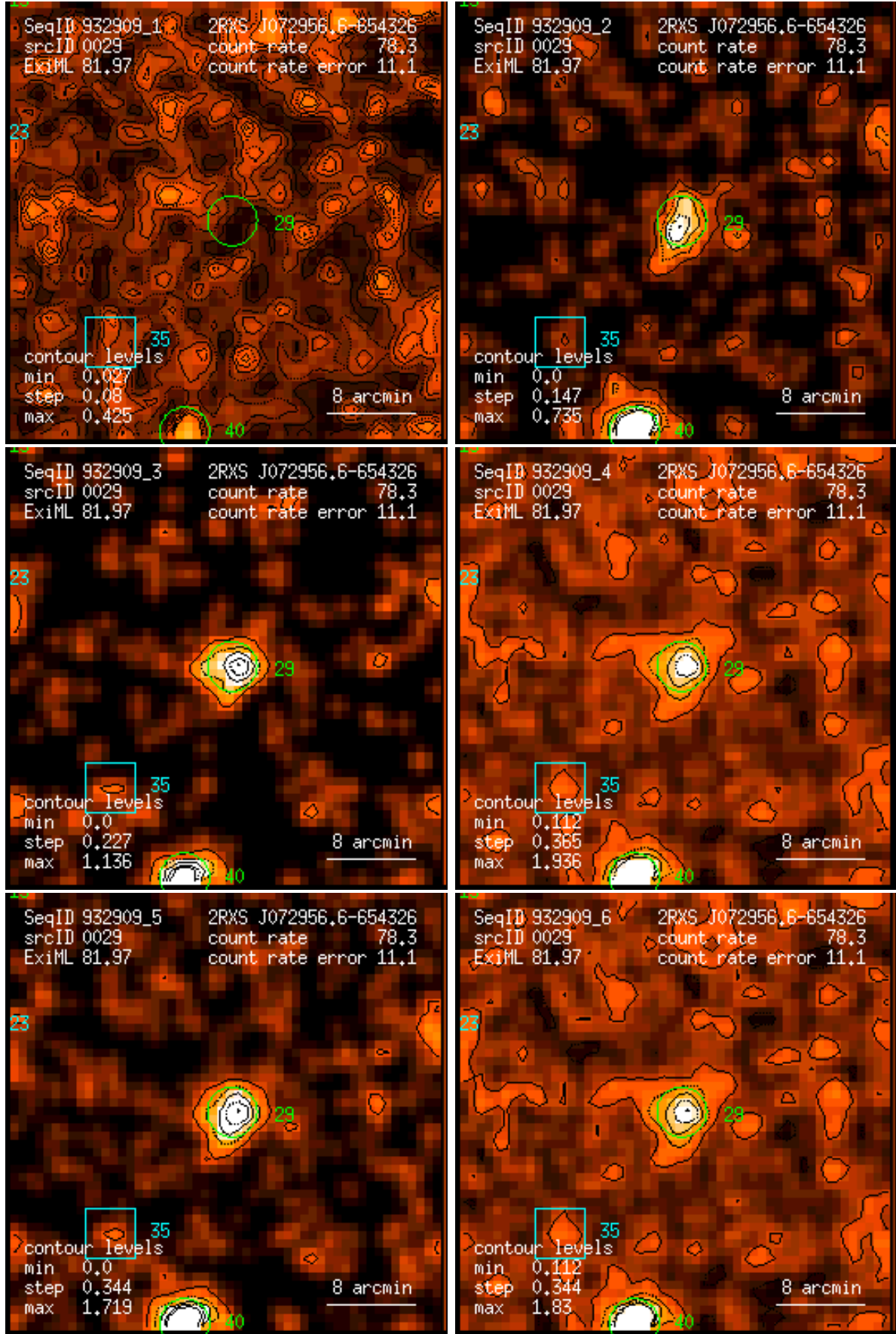
Figure 29: RASS 932909: detection 0029: band rate images, Gaussian filter: (1) PSPC channels 11 – 41, (2) 52 – 90, (3) 91 – 201, (4) 11 – 235, (5) 52 – 201, (6) 11 – 201. Broad band rates in counts/ks. Band rate contour levels in counts/ks/arcmin 2 .
