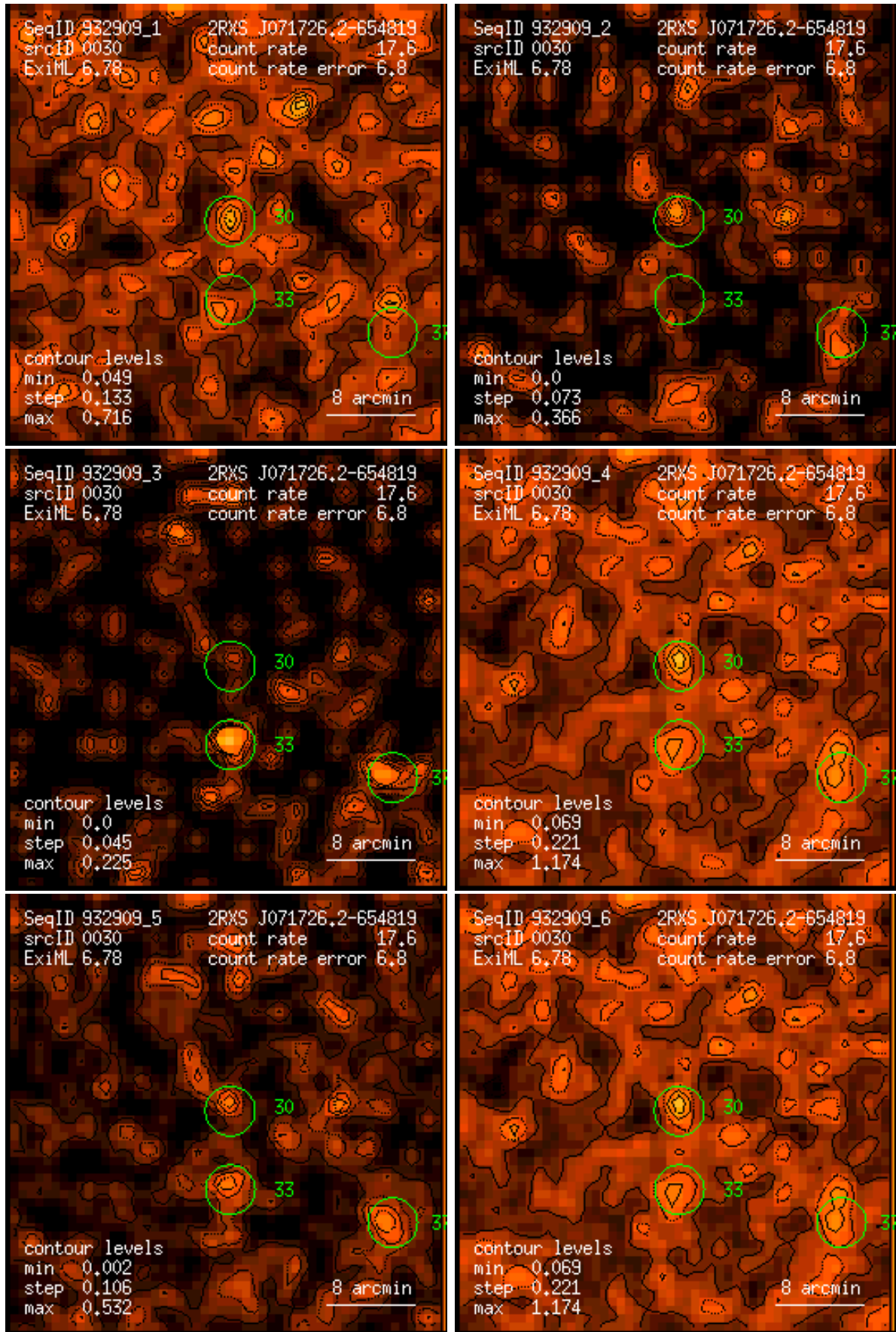
Figure 30: RASS 932909: detection 0030: band rate images, Gaussian filter: (1) PSPC channels 11 – 41, (2) 52 – 90, (3) 91 – 201, (4) 11 – 235, (5) 52 – 201, (6) 11 – 201. Broad band rates in counts/ks. Band rate contour levels in counts/ks/arcmin 2 .
