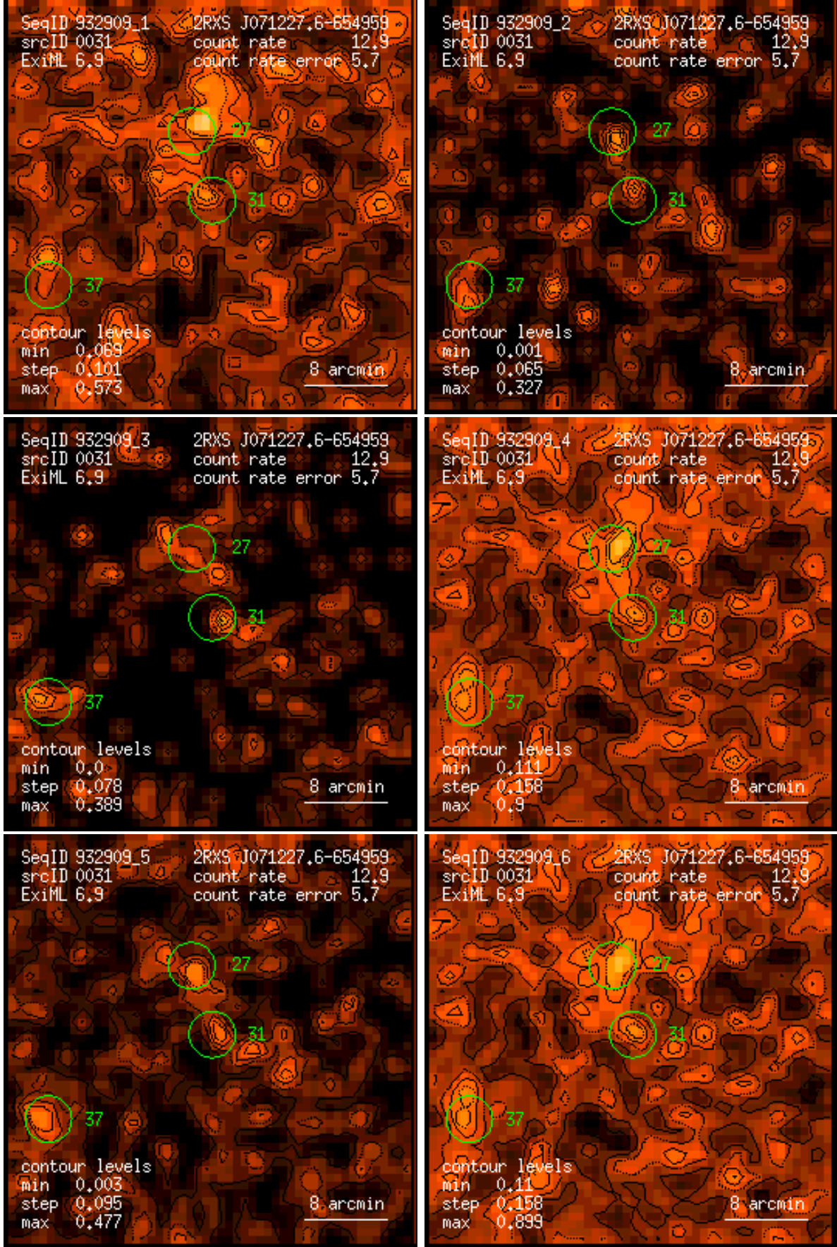
Figure 31: RASS 932909: detection 0031: band rate images, Gaussian filter: (1) PSPC channels 11 – 41, (2) 52 – 90, (3) 91 – 201, (4) 11 – 235, (5) 52 – 201, (6) 11 – 201. Broad band rates in counts/ks. Band rate contour levels in counts/ks/arcmin 2 .
