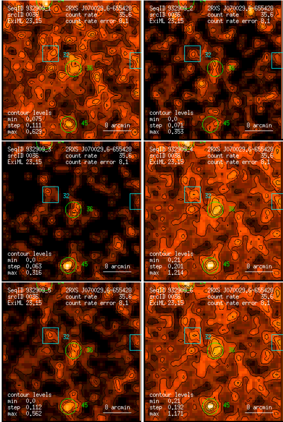
Figure 36: RASS 932909: detection 0036: band rate images, Gaussian filter: (1) PSPC channels 11 – 41, (2) 52 – 90, (3) 91 – 201, (4) 11 – 235, (5) 52 – 201, (6) 11 – 201. Broad band rates in counts/ks. Band rate contour levels in counts/ks/arcmin 2 .
