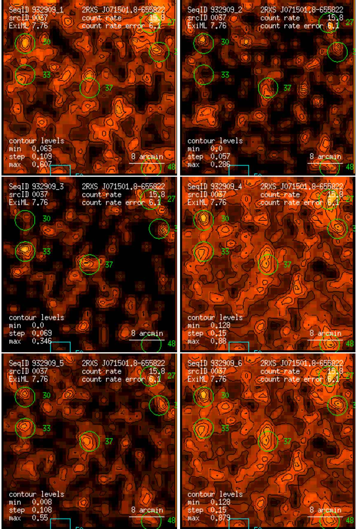
Figure 37: RASS 932909: detection 0037: band rate images, Gaussian filter: (1) PSPC channels 11 – 41, (2) 52 – 90, (3) 91 – 201, (4) 11 – 235, (5) 52 – 201, (6) 11 – 201. Broad band rates in counts/ks. Band rate contour levels in counts/ks/arcmin 2 .
