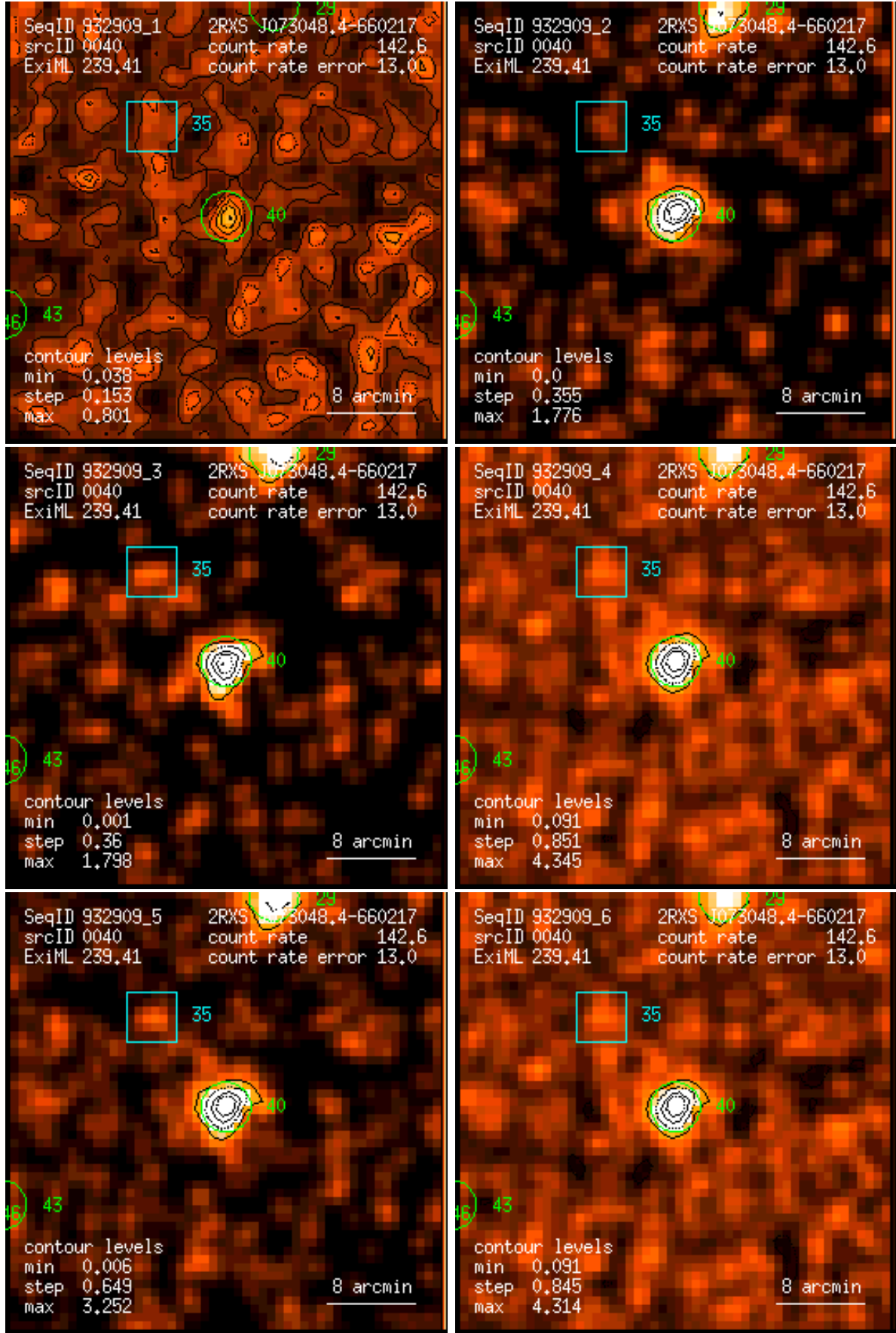
Figure 40: RASS 932909: detection 0040: band rate images, Gaussian filter: (1) PSPC channels 11 – 41, (2) 52 – 90, (3) 91 – 201, (4) 11 – 235, (5) 52 – 201, (6) 11 – 201. Broad band rates in counts/ks. Band rate contour levels in counts/ks/arcmin 2 .
