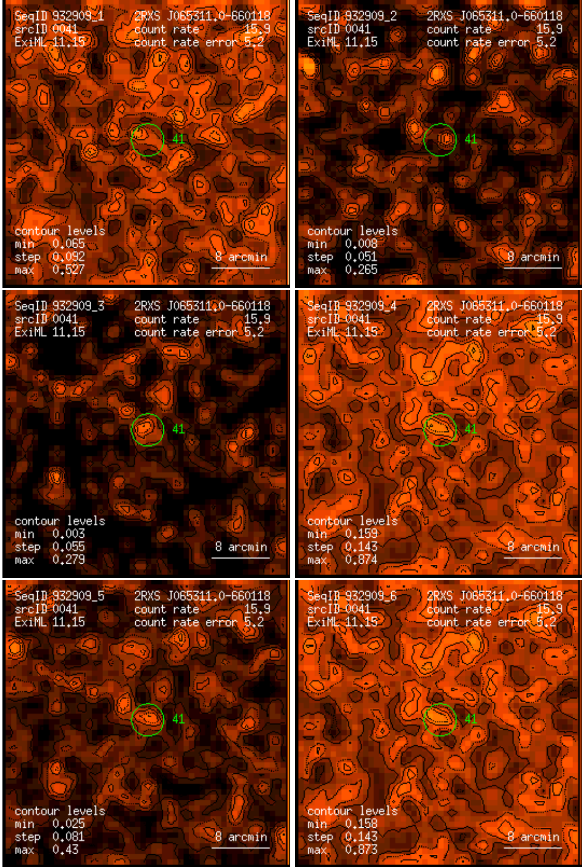
Figure 41: RASS 932909: detection 0041: band rate images, Gaussian filter: (1) PSPC channels 11 – 41, (2) 52 – 90, (3) 91 – 201, (4) 11 – 235, (5) 52 – 201, (6) 11 – 201. Broad band rates in counts/ks. Band rate contour levels in counts/ks/arcmin 2 .
