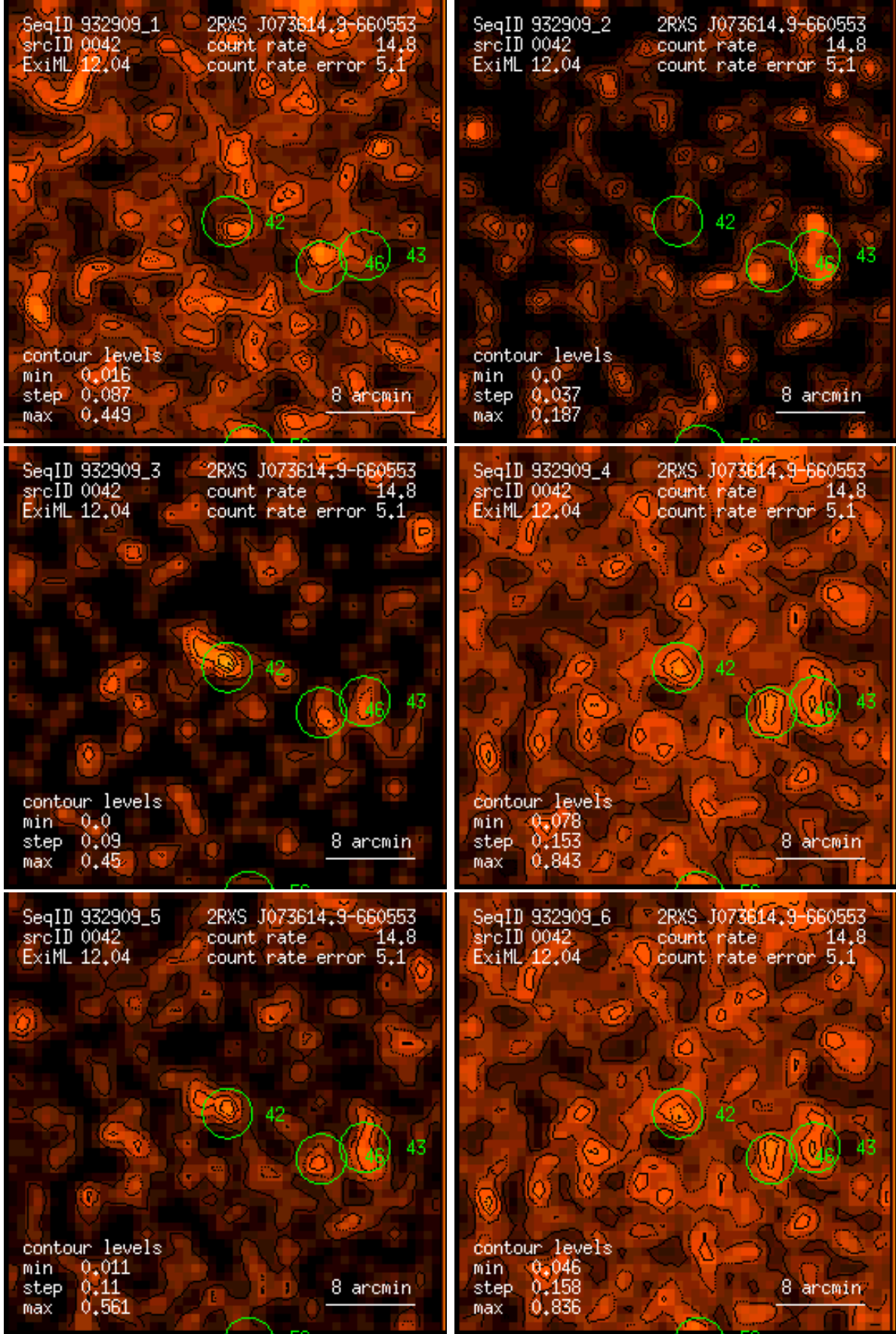
Figure 42: RASS 932909: detection 0042: band rate images, Gaussian filter: (1) PSPC channels 11 – 41, (2) 52 – 90, (3) 91 – 201, (4) 11 – 235, (5) 52 – 201, (6) 11 – 201. Broad band rates in counts/ks. Band rate contour levels in counts/ks/arcmin 2 .
