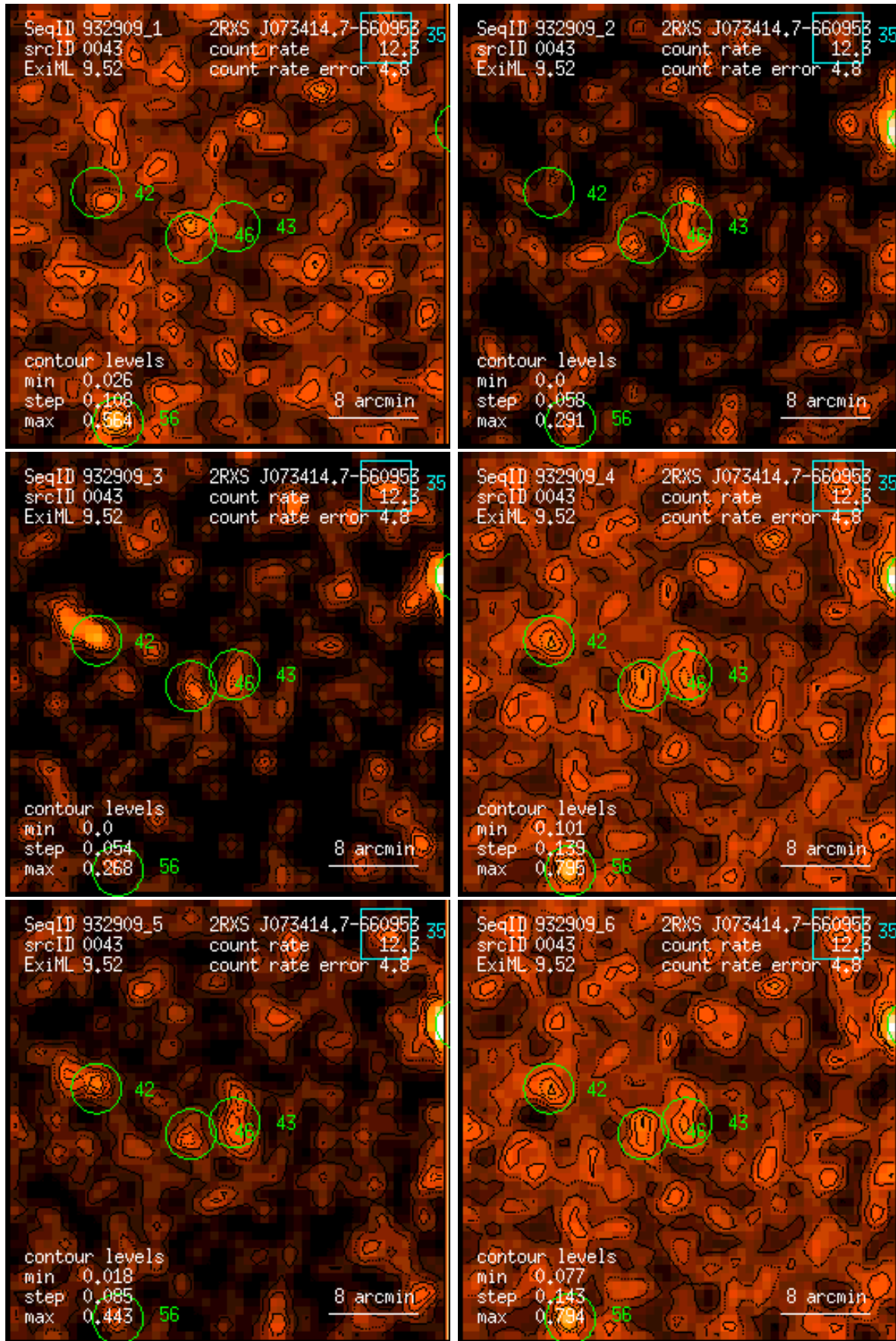
Figure 43: RASS 932909: detection 0043: band rate images, Gaussian filter: (1) PSPC channels 11 – 41, (2) 52 – 90, (3) 91 – 201, (4) 11 – 235, (5) 52 – 201, (6) 11 – 201. Broad band rates in counts/ks. Band rate contour levels in counts/ks/arcmin 2 .
