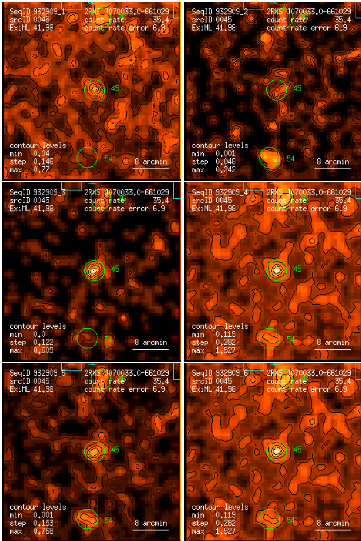
Figure 45: RASS 932909: detection 0045: band rate images, Gaussian filter: (1) PSPC channels 11 – 41, (2) 52 – 90, (3) 91 – 201, (4) 11 – 235, (5) 52 – 201, (6) 11 – 201. Broad band rates in counts/ks. Band rate contour levels in counts/ks/arcmin 2 .
