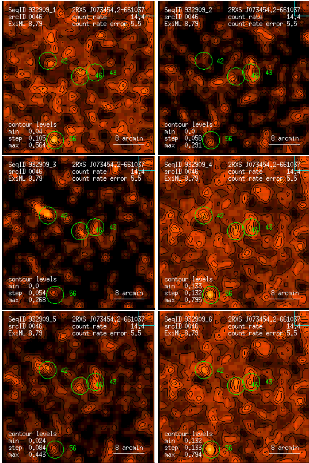
Figure 46: RASS 932909: detection 0046: band rate images, Gaussian filter: (1) PSPC channels 11 – 41, (2) 52 – 90, (3) 91 – 201, (4) 11 – 235, (5) 52 – 201, (6) 11 – 201. Broad band rates in counts/ks. Band rate contour levels in counts/ks/arcmin 2 .
