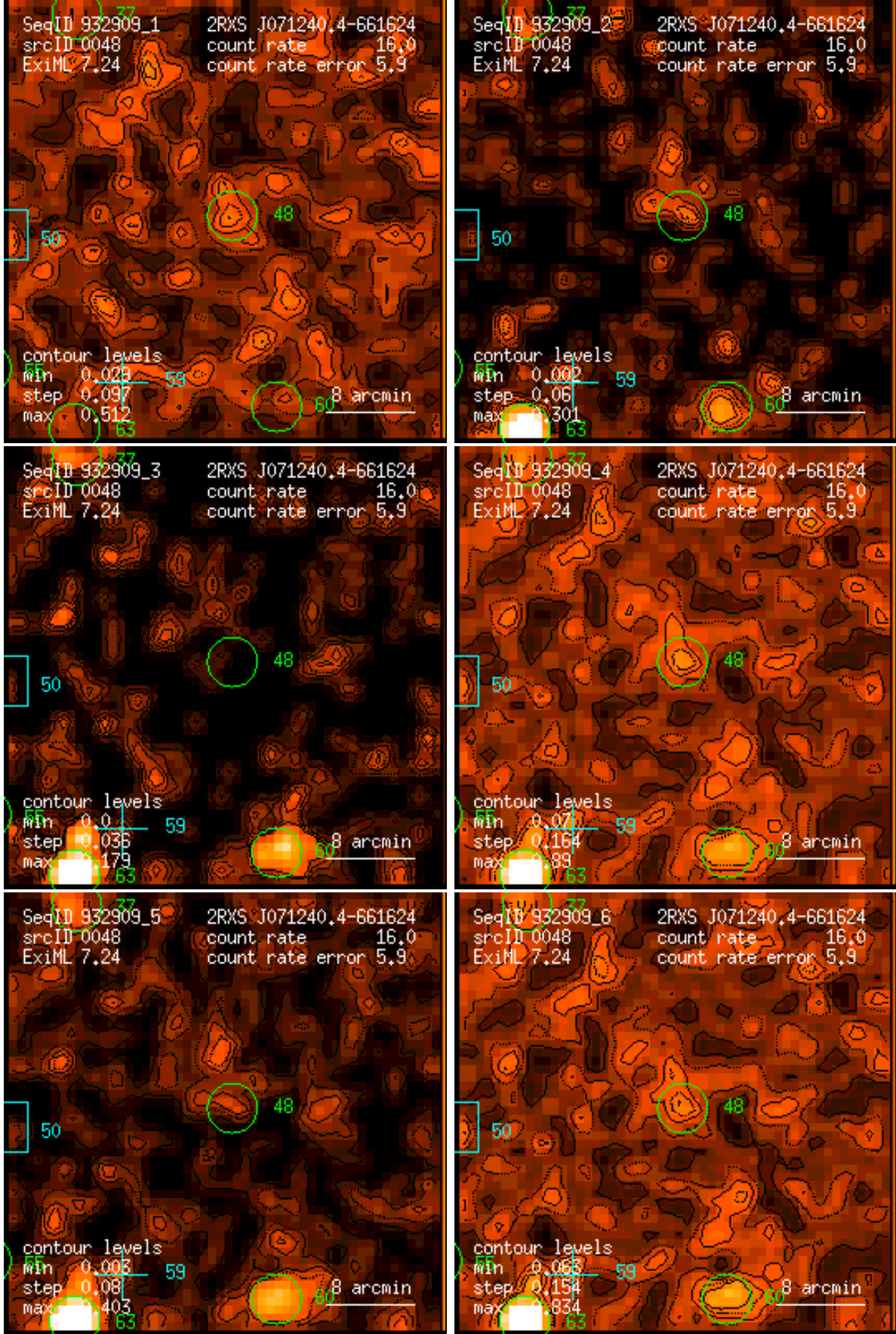
Figure 48: RASS 932909: detection 0048: band rate images, Gaussian filter: (1) PSPC channels 11 – 41, (2) 52 – 90, (3) 91 – 201, (4) 11 – 235, (5) 52 – 201, (6) 11 – 201. Broad band rates in counts/ks. Band rate contour levels in counts/ks/arcmin 2 .
