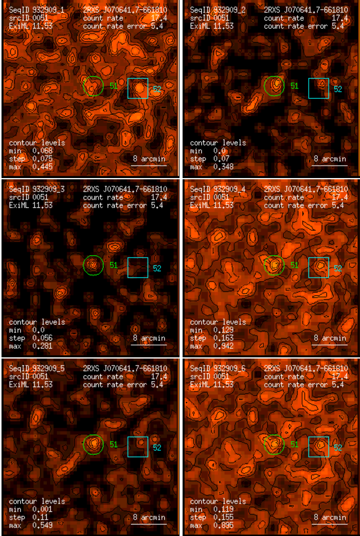
Figure 51: RASS 932909: detection 0051: band rate images, Gaussian filter: (1) PSPC channels 11 – 41, (2) 52 – 90, (3) 91 – 201, (4) 11 – 235, (5) 52 – 201, (6) 11 – 201. Broad band rates in counts/ks. Band rate contour levels in counts/ks/arcmin 2 .
