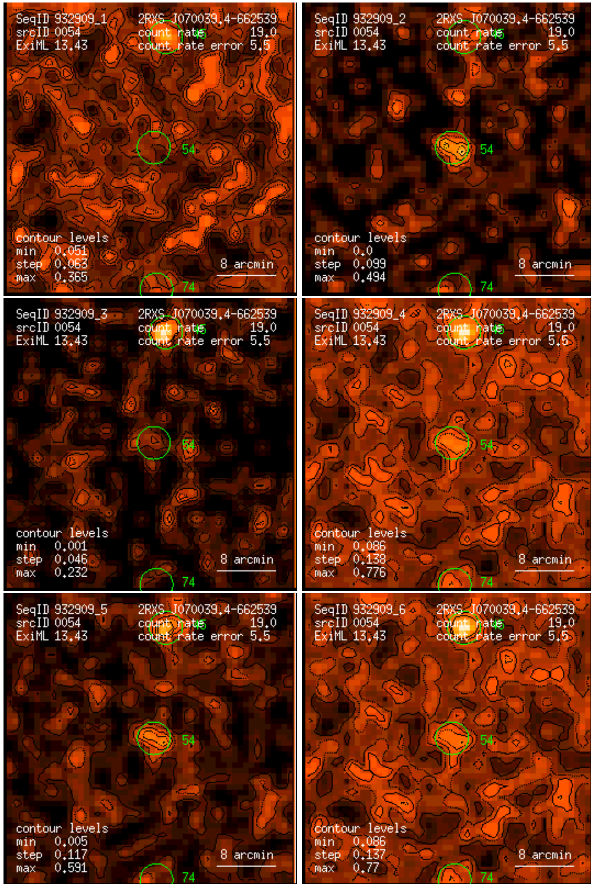
Figure 54: RASS 932909: detection 0054: band rate images, Gaussian filter: (1) PSPC channels 11 – 41, (2) 52 – 90, (3) 91 – 201, (4) 11 – 235, (5) 52 – 201, (6) 11 – 201. Broad band rates in counts/ks. Band rate contour levels in counts/ks/arcmin 2 .
