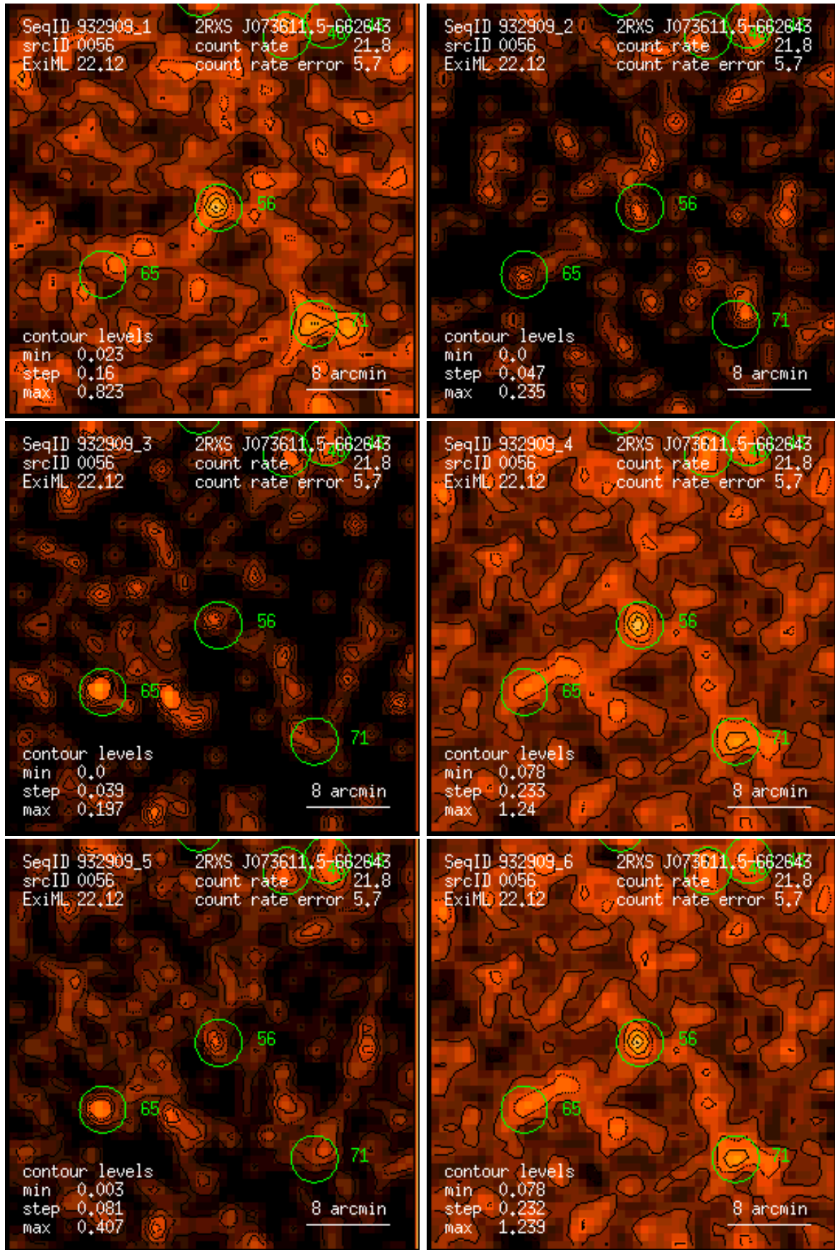
Figure 56: RASS 932909: detection 0056: band rate images, Gaussian filter: (1) PSPC channels 11 – 41, (2) 52 – 90, (3) 91 – 201, (4) 11 – 235, (5) 52 – 201, (6) 11 – 201. Broad band rates in counts/ks. Band rate contour levels in counts/ks/arcmin 2 .
