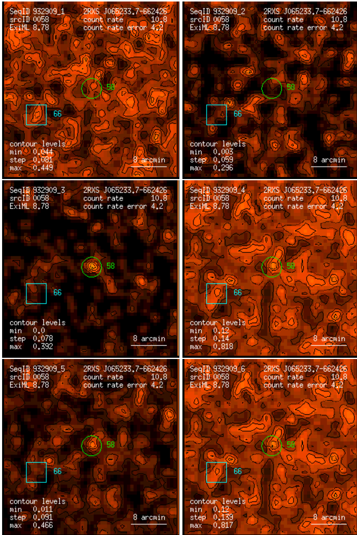
Figure 58: RASS 932909: detection 0058: band rate images, Gaussian filter: (1) PSPC channels 11 – 41, (2) 52 – 90, (3) 91 – 201, (4) 11 – 235, (5) 52 – 201, (6) 11 – 201. Broad band rates in counts/ks. Band rate contour levels in counts/ks/arcmin 2 .
