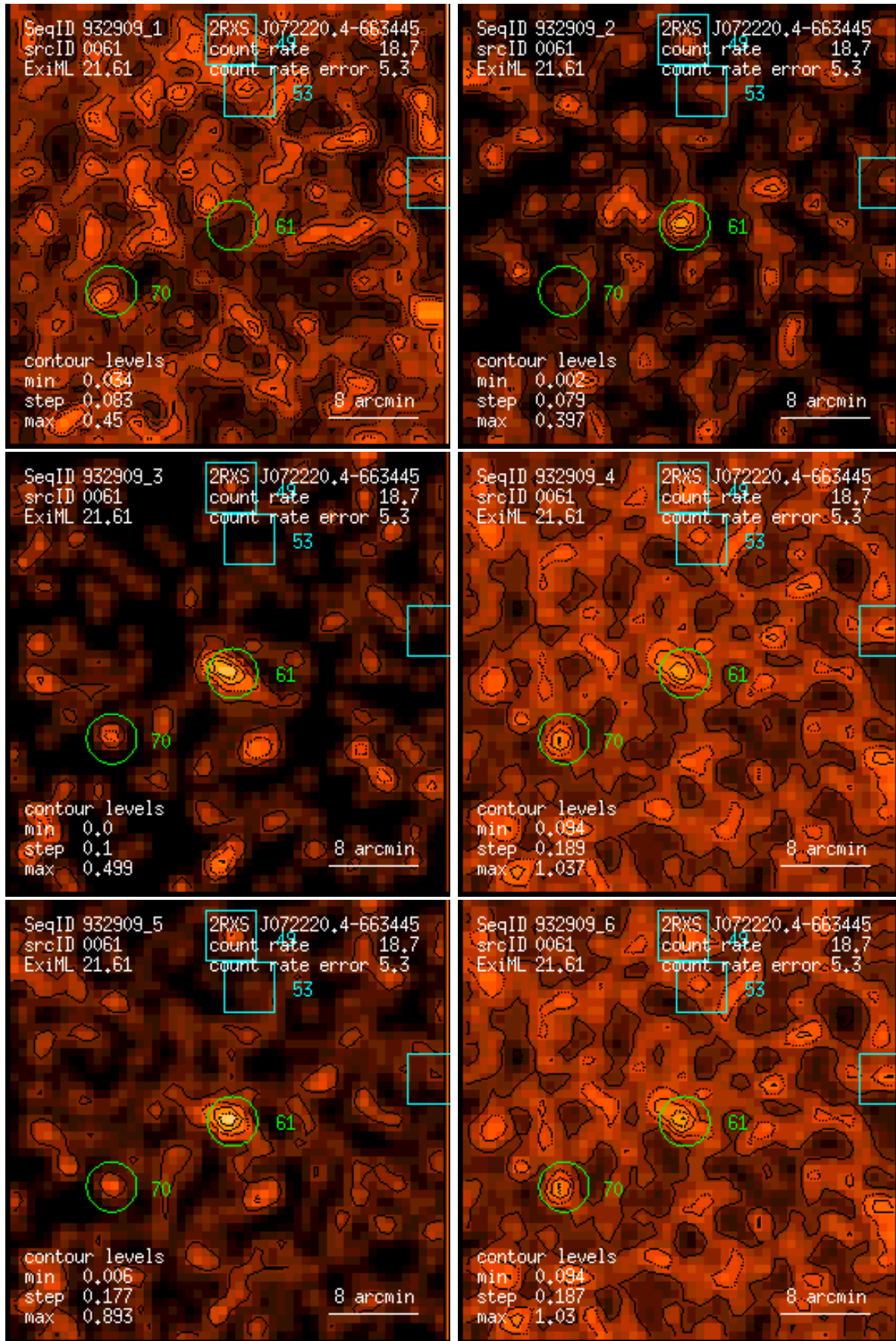
Figure 61: RASS 932909: detection 0061: band rate images, Gaussian filter: (1) PSPC channels 11 – 41, (2) 52 – 90, (3) 91 – 201, (4) 11 – 235, (5) 52 – 201, (6) 11 – 201. Broad band rates in counts/ks. Band rate contour levels in counts/ks/arcmin 2 .
