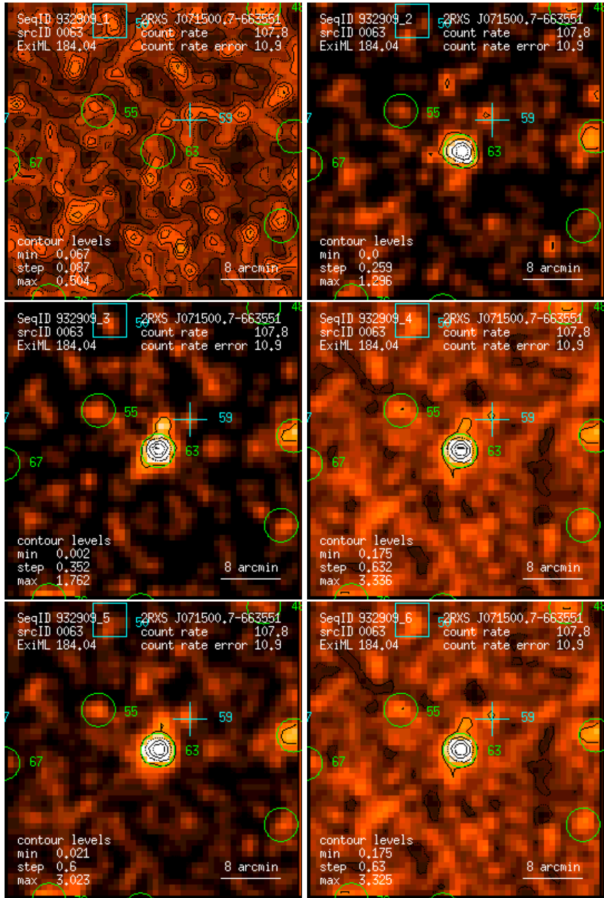
Figure 63: RASS 932909: detection 0063: band rate images, Gaussian filter: (1) PSPC channels 11 – 41, (2) 52 – 90, (3) 91 – 201, (4) 11 – 235, (5) 52 – 201, (6) 11 – 201. Broad band rates in counts/ks. Band rate contour levels in counts/ks/arcmin 2 .
