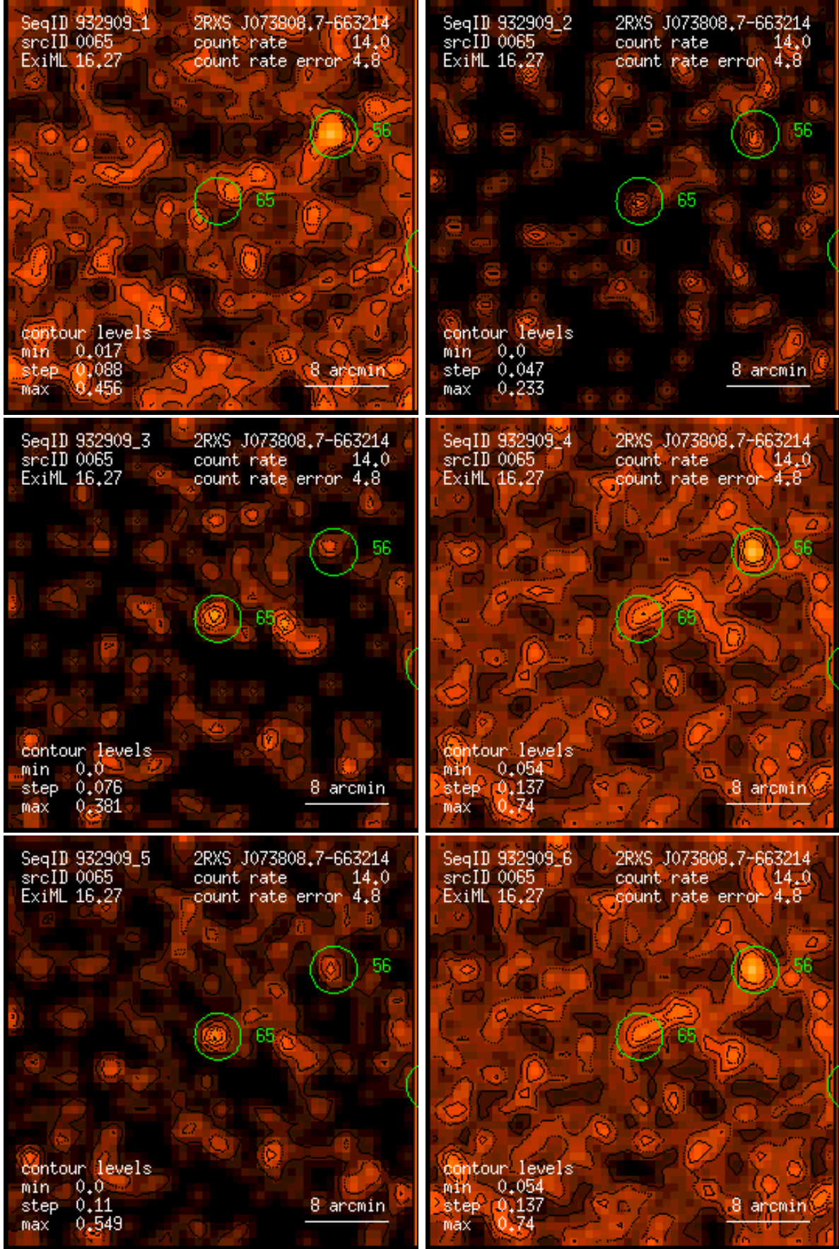
Figure 65: RASS 932909: detection 0065: band rate images, Gaussian filter: (1) PSPC channels 11 – 41, (2) 52 – 90, (3) 91 – 201, (4) 11 – 235, (5) 52 – 201, (6) 11 – 201. Broad band rates in counts/ks. Band rate contour levels in counts/ks/arcmin 2 .
