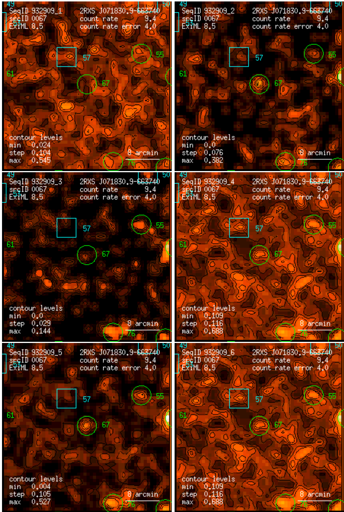
Figure 67: RASS 932909: detection 0067: band rate images, Gaussian filter: (1) PSPC channels 11 – 41, (2) 52 – 90, (3) 91 – 201, (4) 11 – 235, (5) 52 – 201, (6) 11 – 201. Broad band rates in counts/ks. Band rate contour levels in counts/ks/arcmin 2 .
