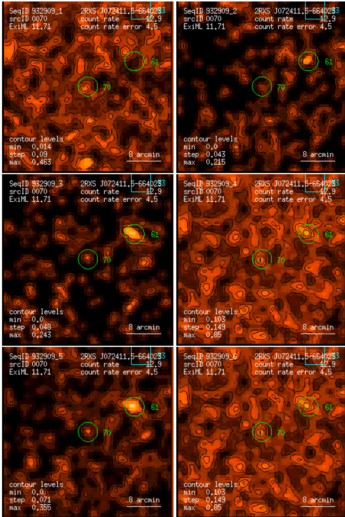
Figure 70: RASS 932909: detection 0070: band rate images, Gaussian filter: (1) PSPC channels 11 – 41, (2) 52 – 90, (3) 91 – 201, (4) 11 – 235, (5) 52 – 201, (6) 11 – 201. Broad band rates in counts/ks. Band rate contour levels in counts/ks/arcmin 2 .
