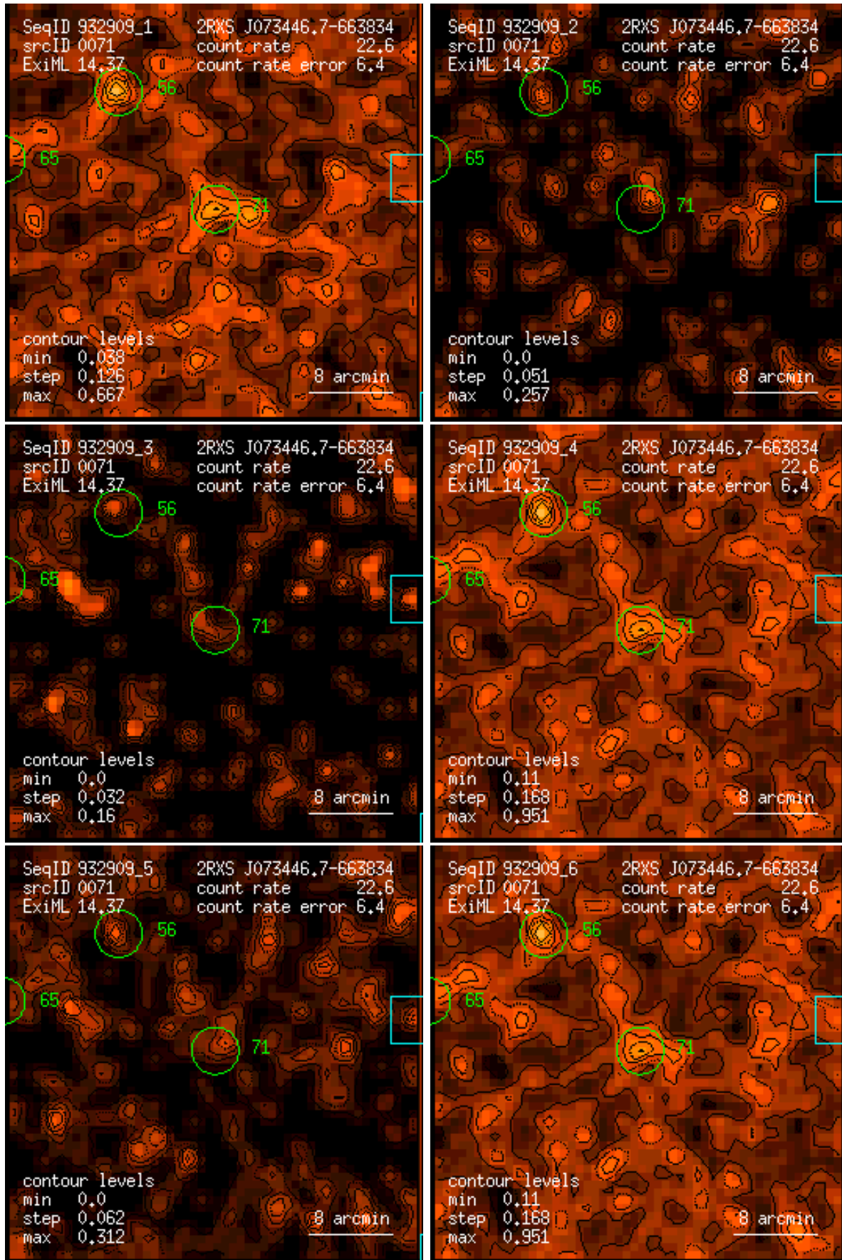
Figure 71: RASS 932909: detection 0071: band rate images, Gaussian filter: (1) PSPC channels 11 – 41, (2) 52 – 90, (3) 91 – 201, (4) 11 – 235, (5) 52 – 201, (6) 11 – 201. Broad band rates in counts/ks. Band rate contour levels in counts/ks/arcmin 2 .
