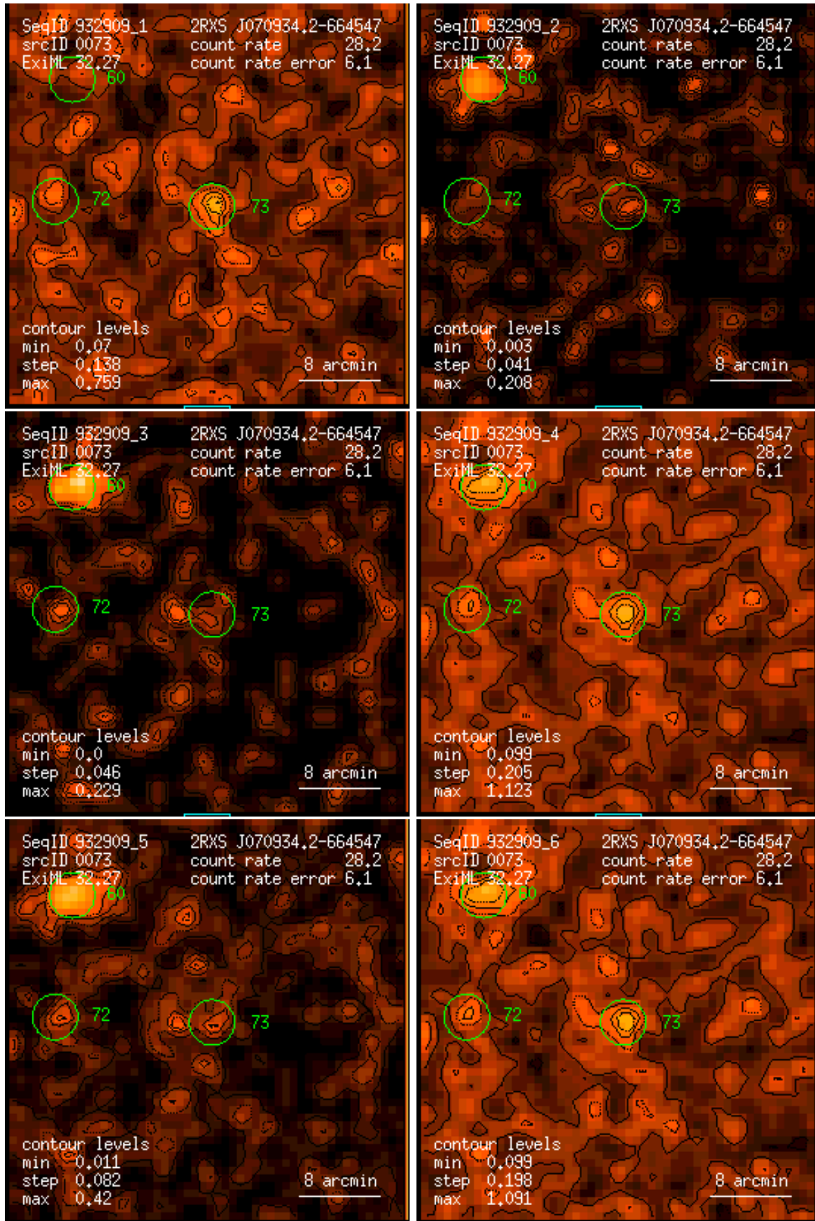
Figure 73: RASS 932909: detection 0073: band rate images, Gaussian filter: (1) PSPC channels 11 – 41, (2) 52 – 90, (3) 91 – 201, (4) 11 – 235, (5) 52 – 201, (6) 11 – 201. Broad band rates in counts/ks. Band rate contour levels in counts/ks/arcmin 2 .
