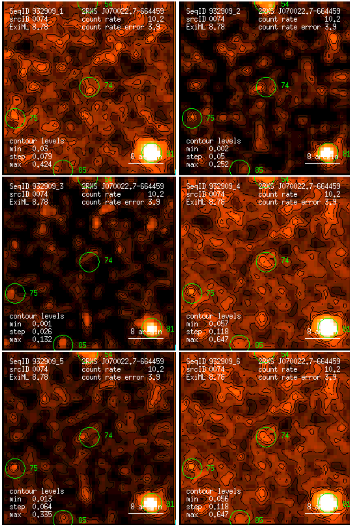
Figure 74: RASS 932909: detection 0074: band rate images, Gaussian filter: (1) PSPC channels 11 – 41, (2) 52 – 90, (3) 91 – 201, (4) 11 – 235, (5) 52 – 201, (6) 11 – 201. Broad band rates in counts/ks. Band rate contour levels in counts/ks/arcmin 2 .
